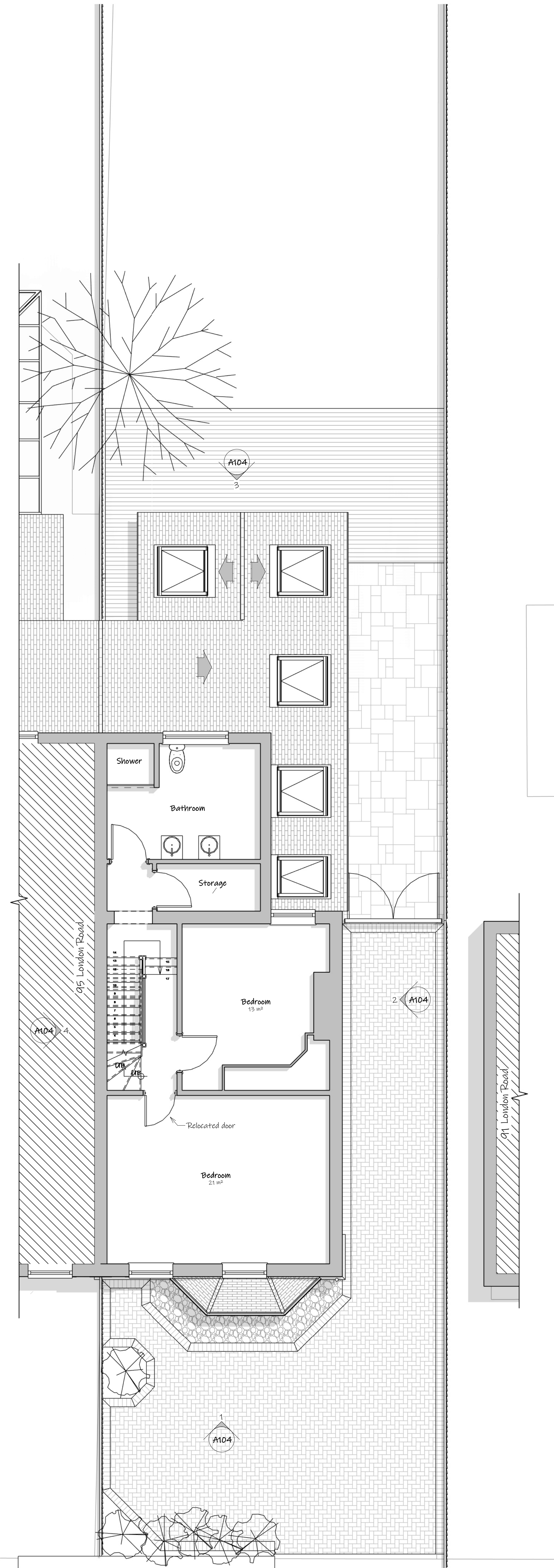
2 Proposed First Floor 1:50
