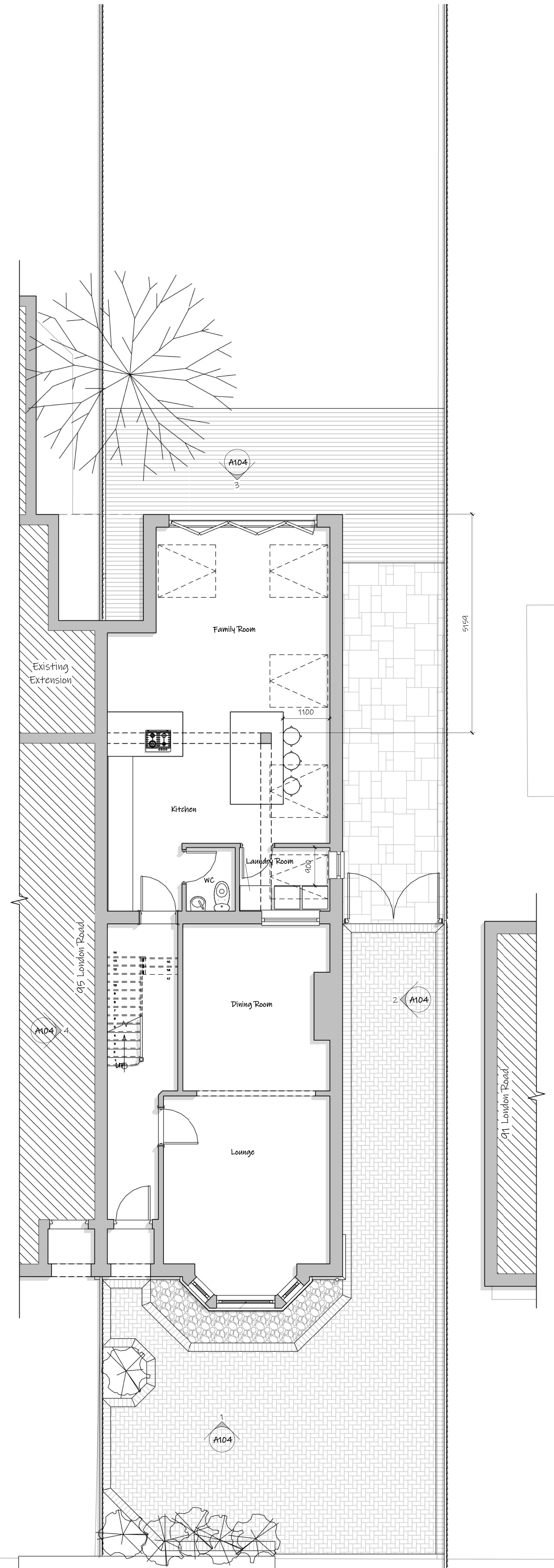
1 Proposed Ground Floor 1:50
