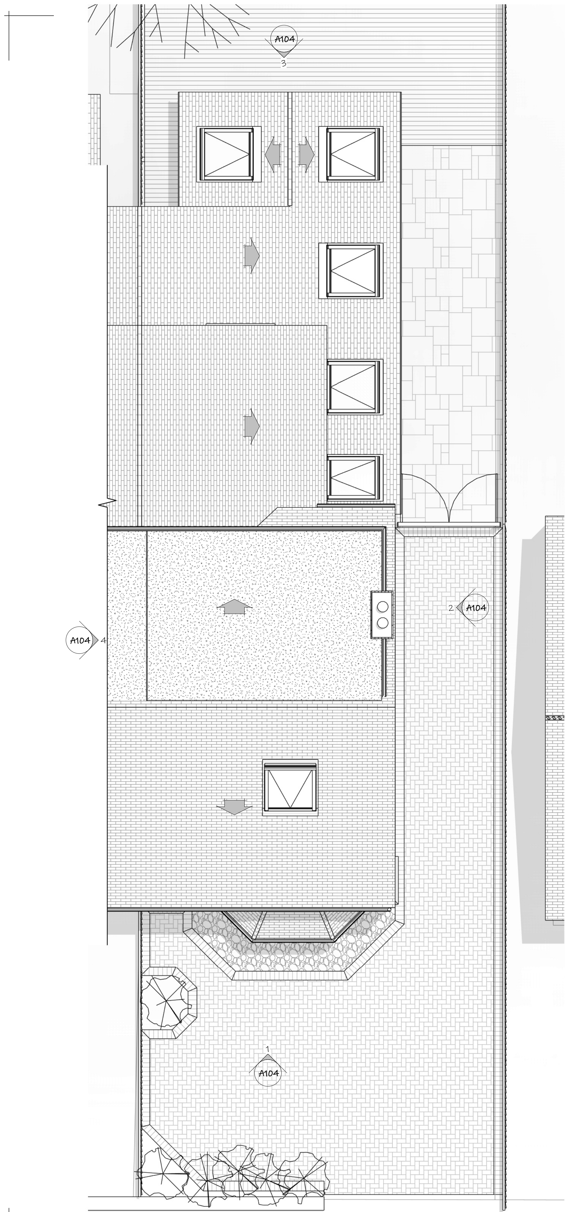
1 Proposed Roof 1:50
