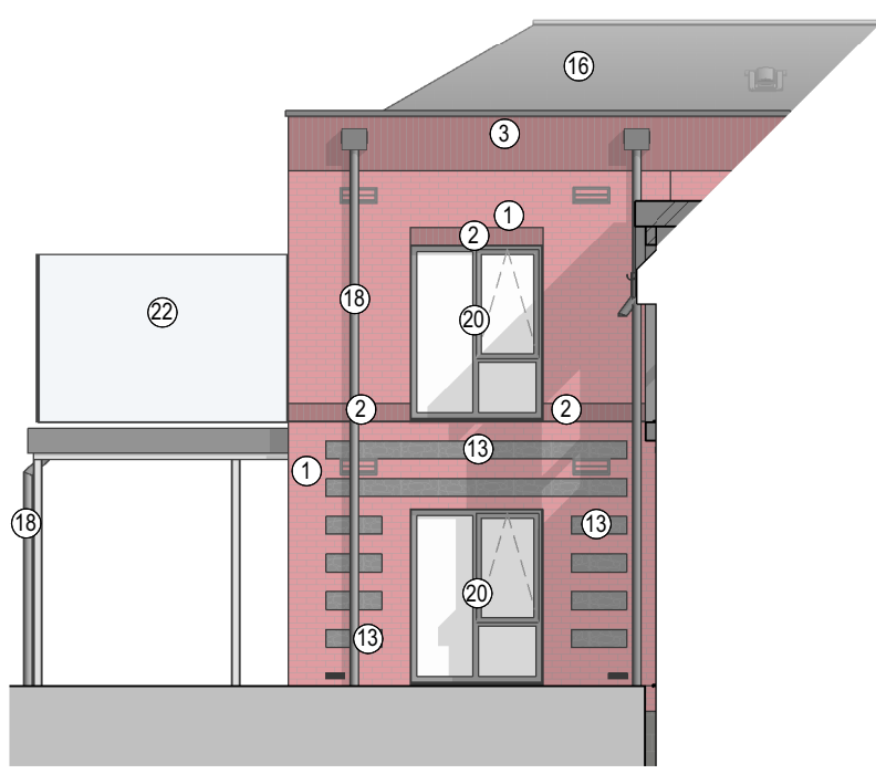
West Elevation (hidden) planning 1:100
