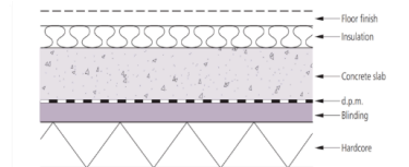
Ground bearing Concrete Slab detail
