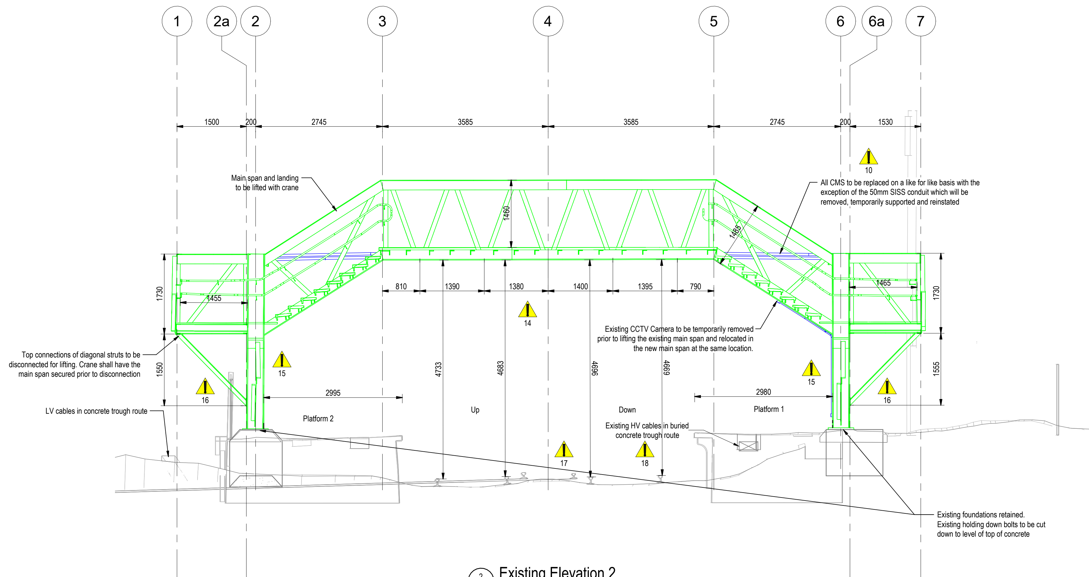
2 Existing Elevation 2 Scale 1 : 50
