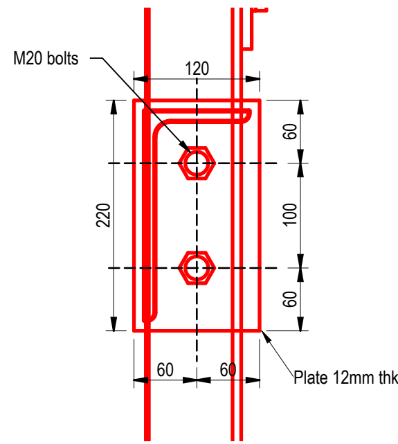
24 002368 Landing Truss - Top Chord to Main Post Scale 1 : 5
