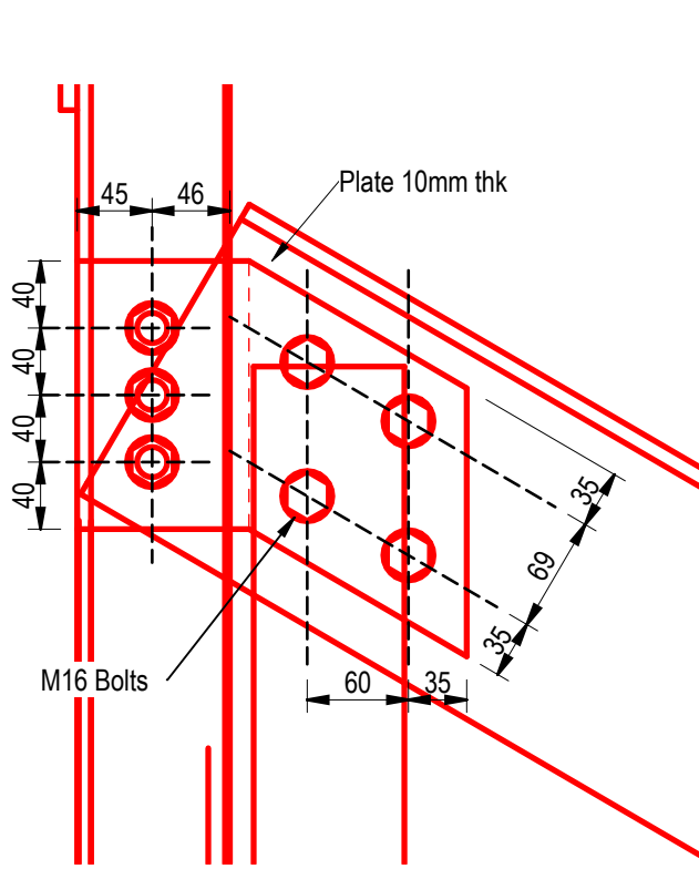
20 002368 Stair Truss - Top to Chord to Main Post Scale 1 : 5
