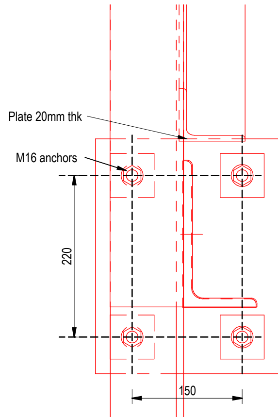
22 002368 Platform 2 Stair Stringer Base Plate Scale 1 : 5
