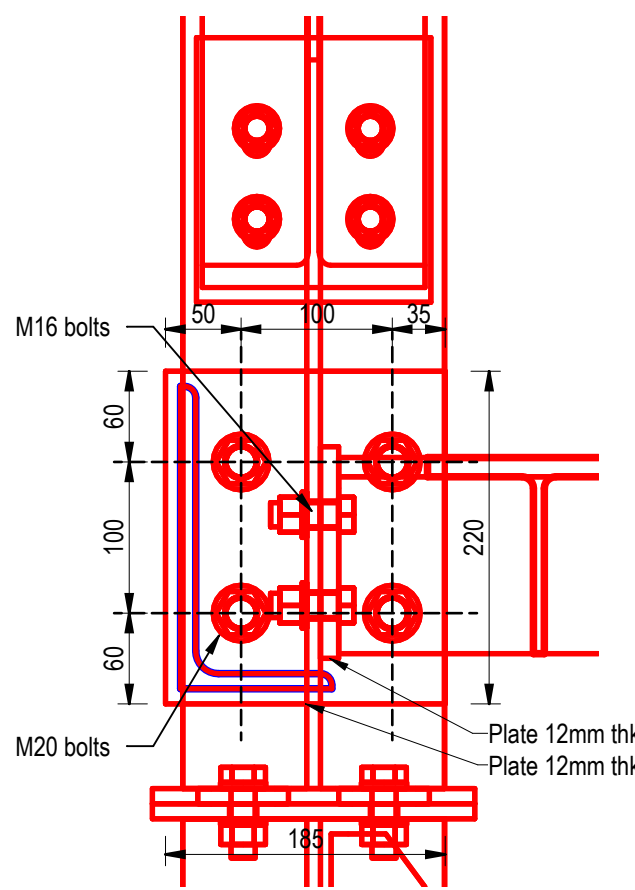
25 002368 Landing Truss - Bottom Chord to Main Post Scale 1 : 5
