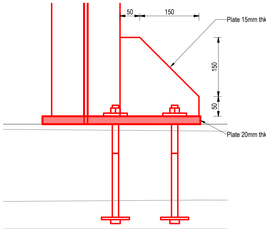
27 002368 Main Post Base Plate - Stiffener Section Scale 1 : 5
