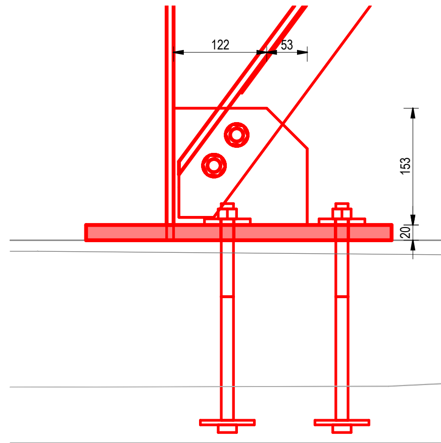
28 002368 Main Post Base Plate - Bracing Section Scale 1 : 5
