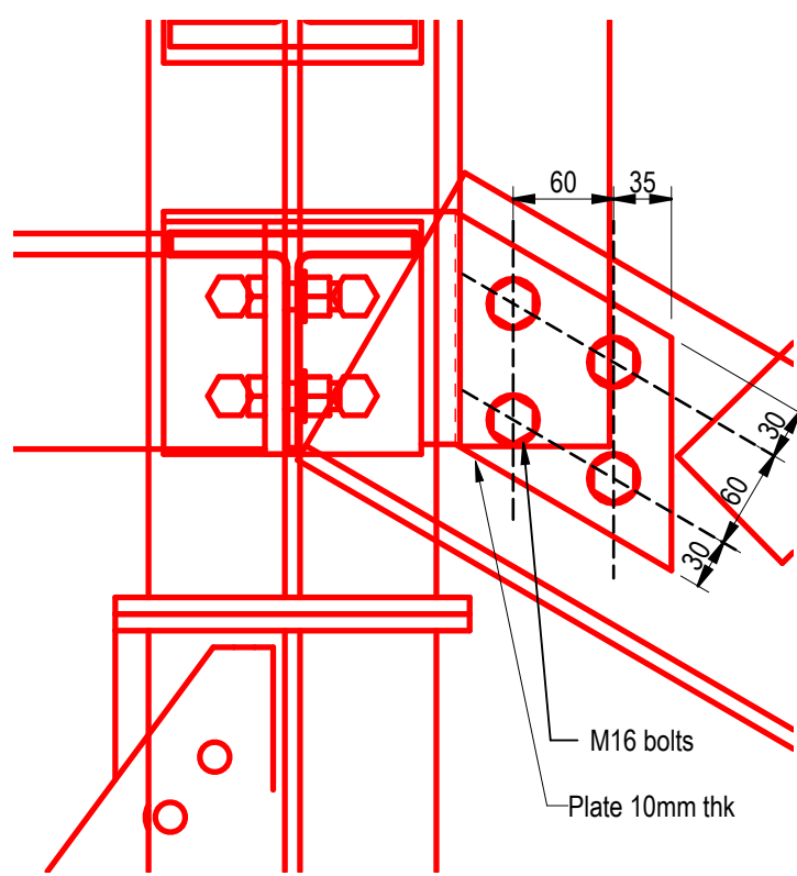
21 002368 Stair Truss - Bottom to Chord to Main Post Scale 1 : 5
