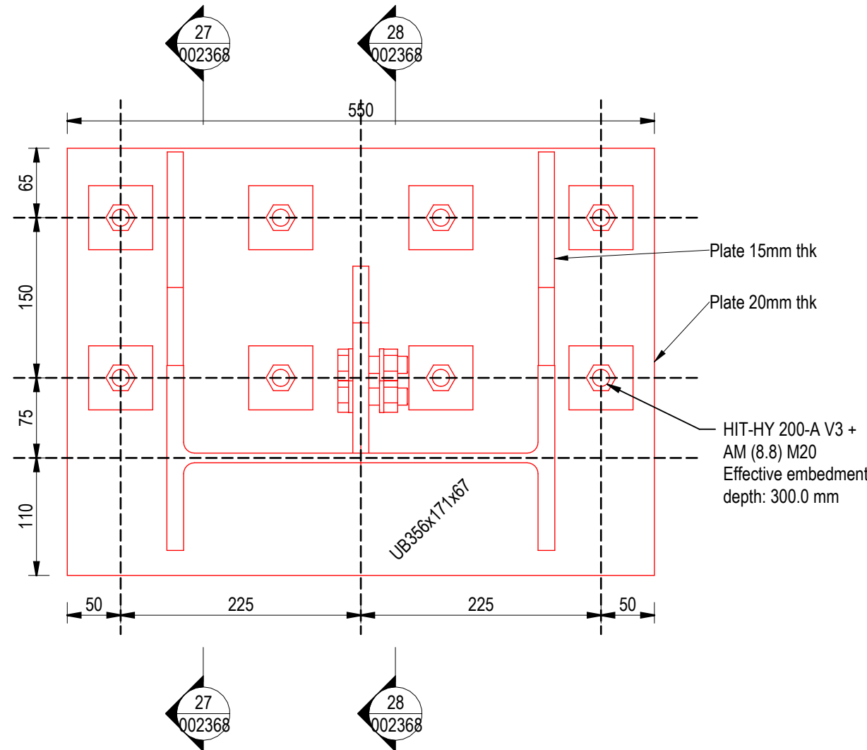
26 002368 Main Post Base Plate Scale 1 : 5
