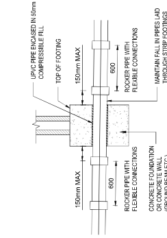
TYPICAL PIPE PENETRATION DETAIL (THROUGH CONCRETE WALL OR FOOTING)
