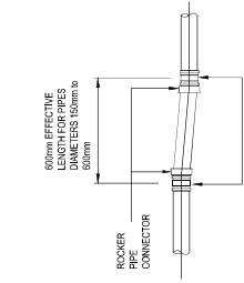
TYPICAL ROCKER PIPE ASSEMBLY
