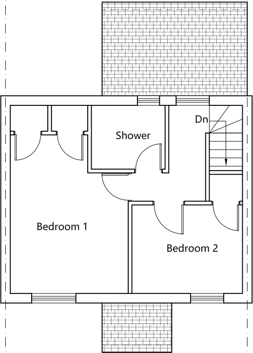
First Floor Plan - No Change
