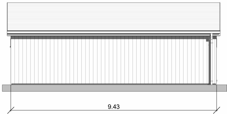
Rear Elevation
