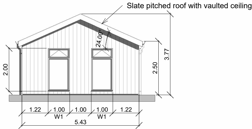
Side Elevation_1
