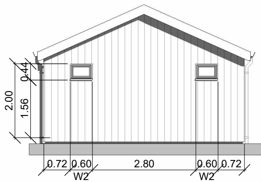
Side Elevation_2
