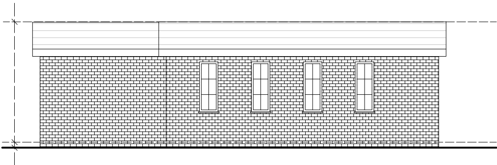
'As EXISTING' REAR ELEVATION
