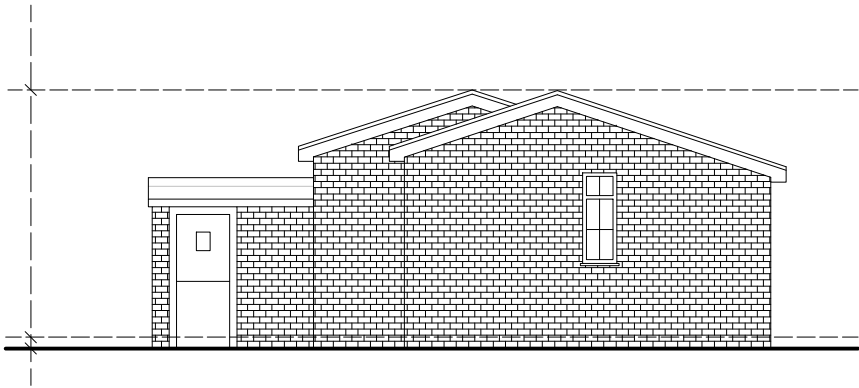
'As EXISTING' SIDE ELEVATION
