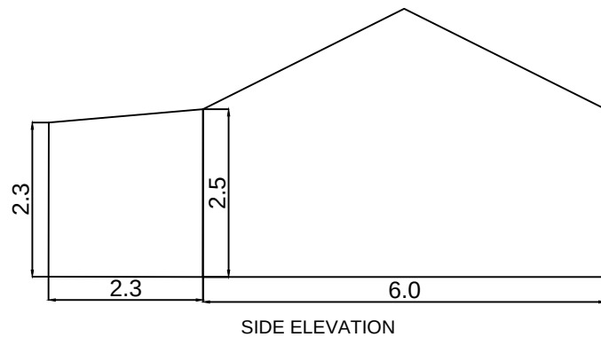
EXISTING ELEVATION
