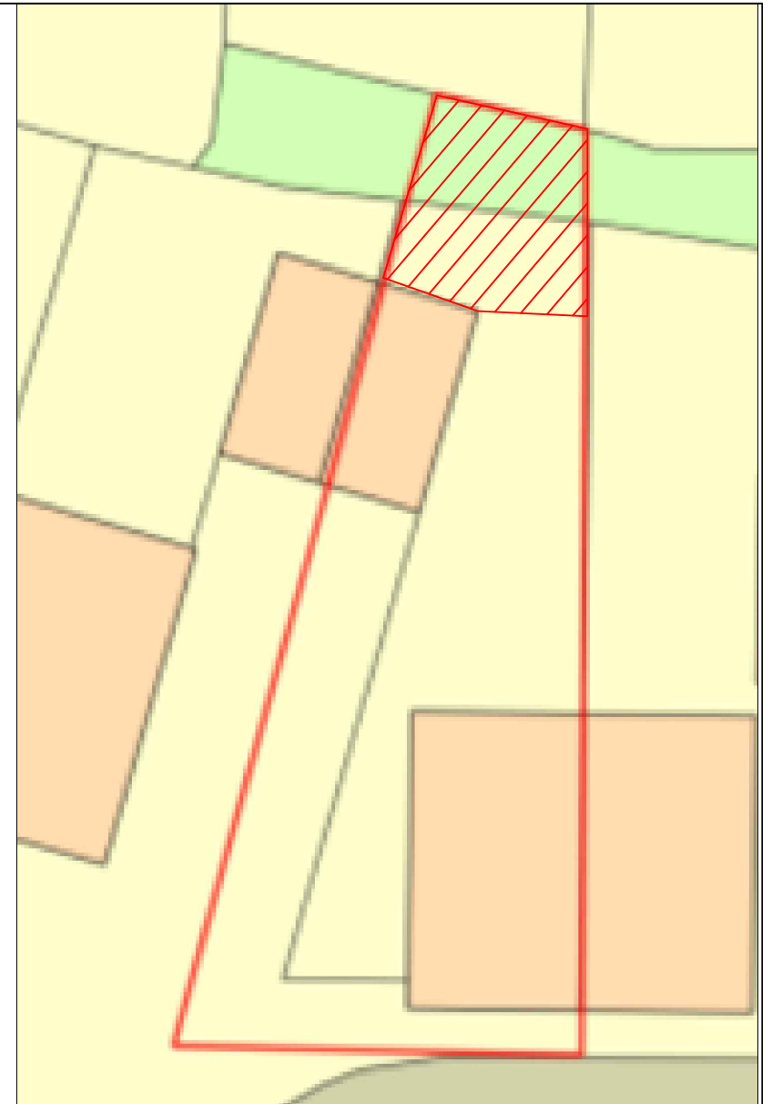
BLOCK PLAN (1:200)
