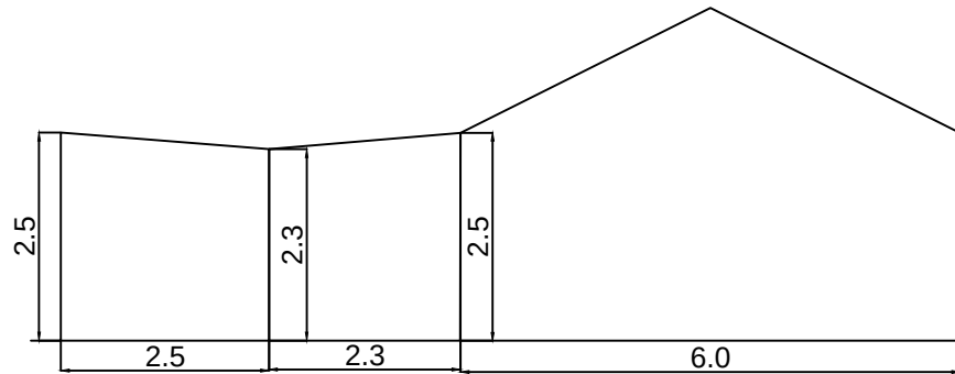
SIDE ELEVATION
