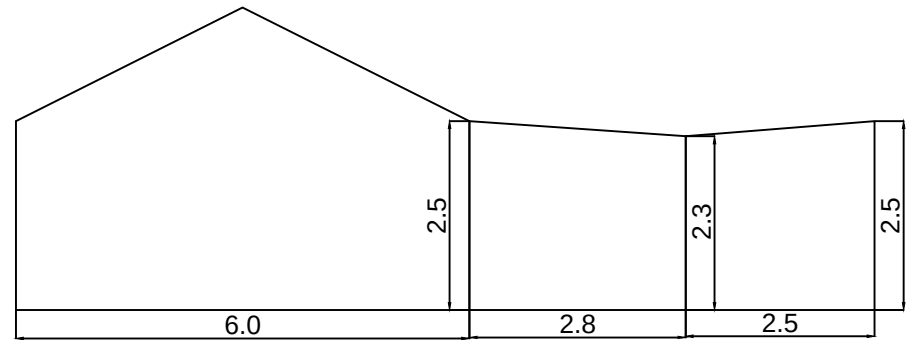
SIDE ELEVATION
