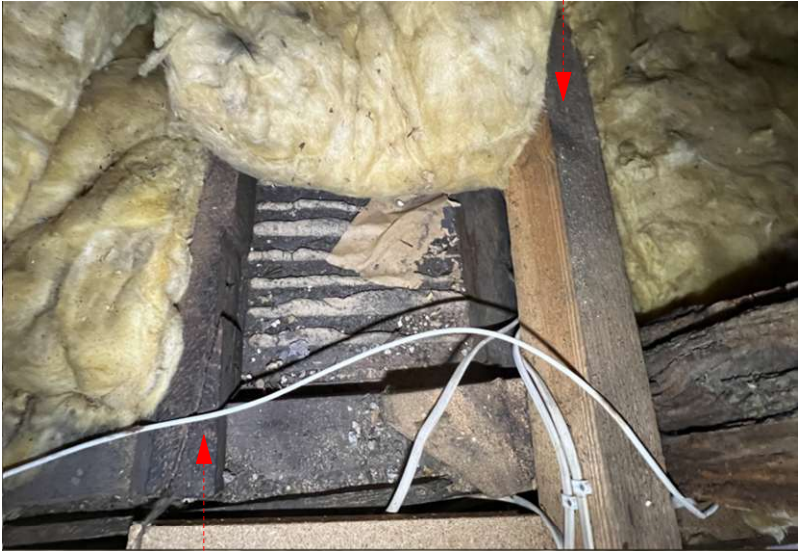
New timbers which sits above existing ceiling with metal straps connecting to rafter
