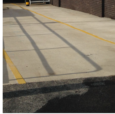
2 Concrete surface to loading bay ramp, pedestrian ramps + Plant slab, brushed finish.
