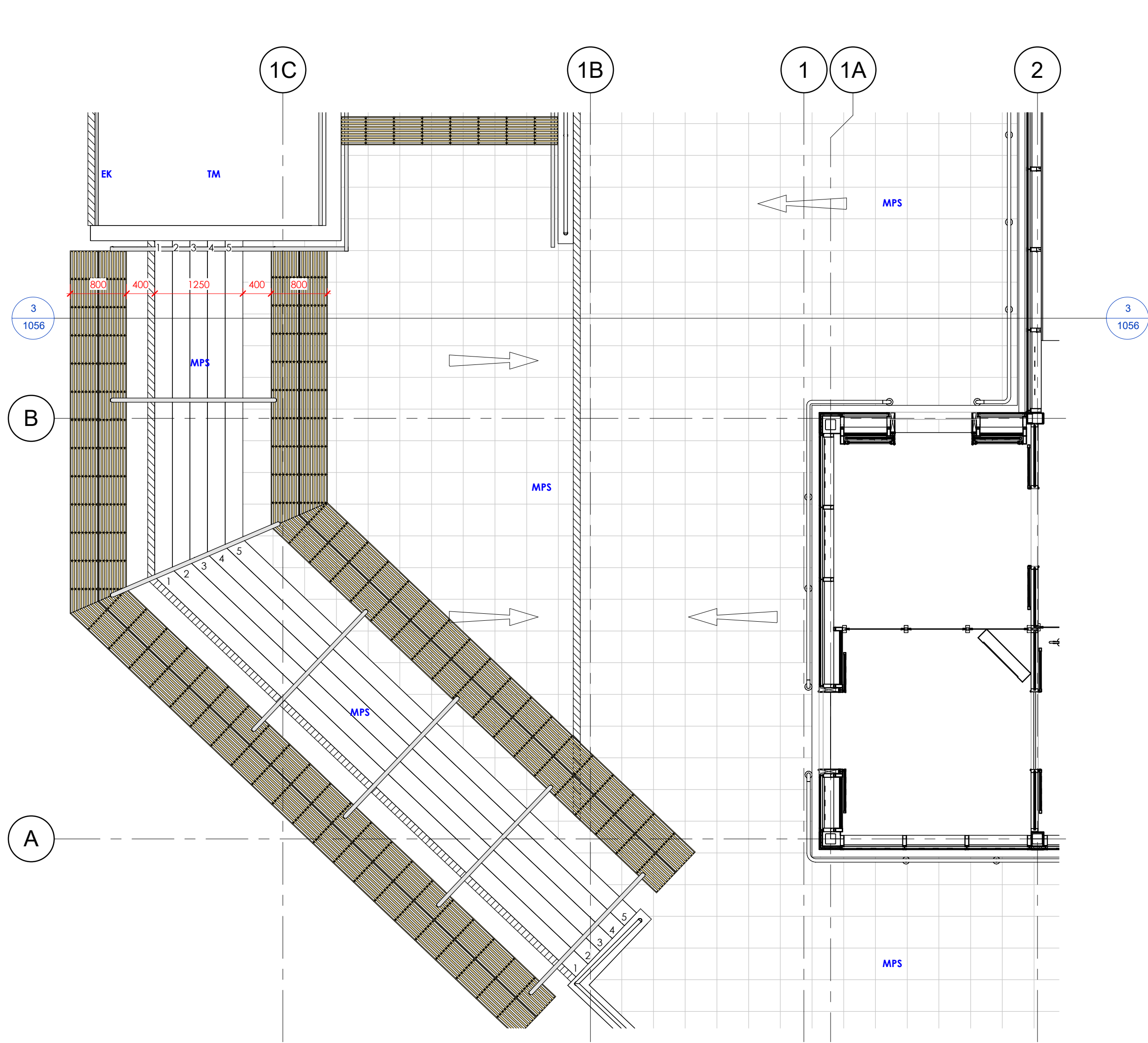
2 ENTRANCE STAIRS PLAN 1 : 50
