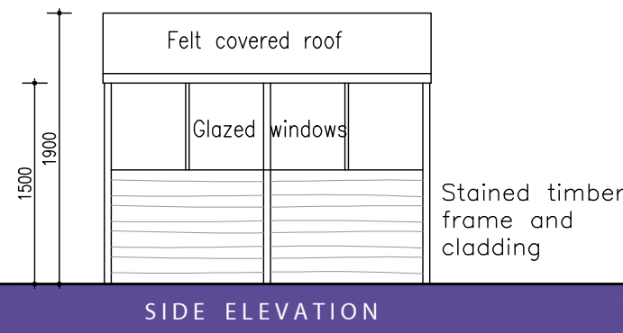
CAR & CYCLE PARKING STANDARD DOCUMENT. Design in accordance with section 4.7- CYCLE PARKING DESIGN
