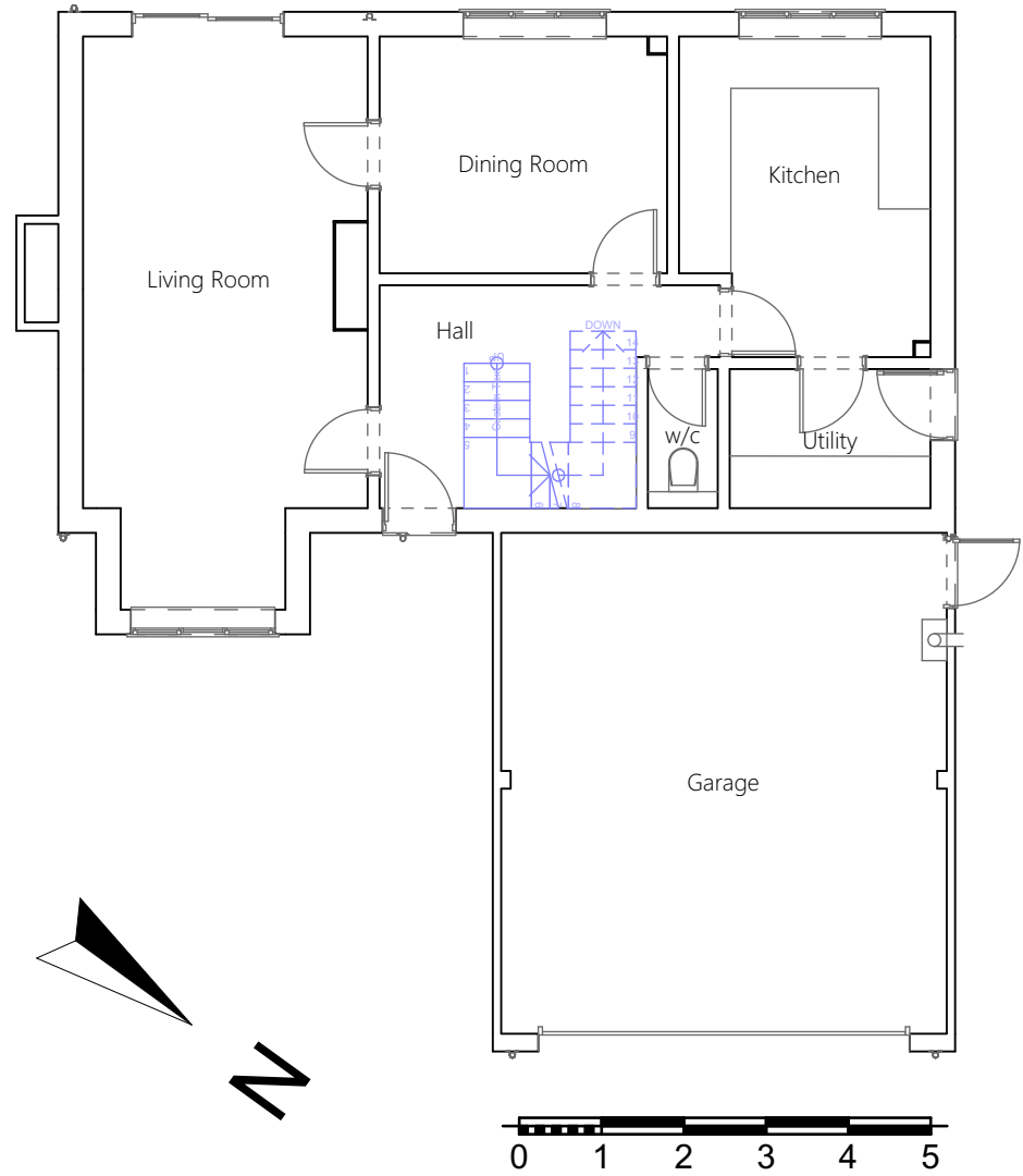
Existing GF-Ground Floor 1:100
