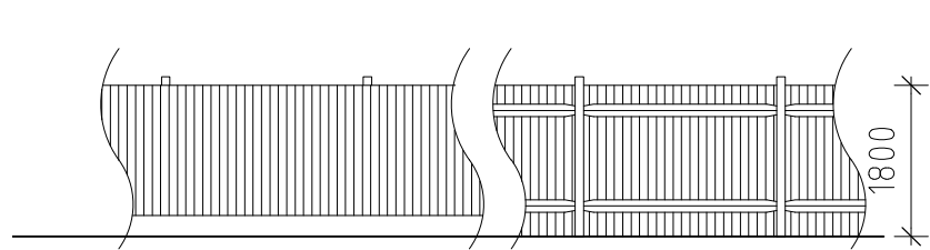
1.8m high Close Board Fence 1:100
