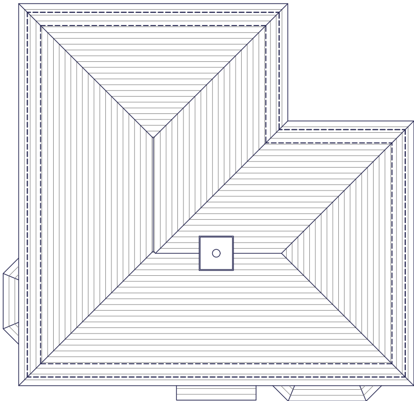
ROOF PLAN
