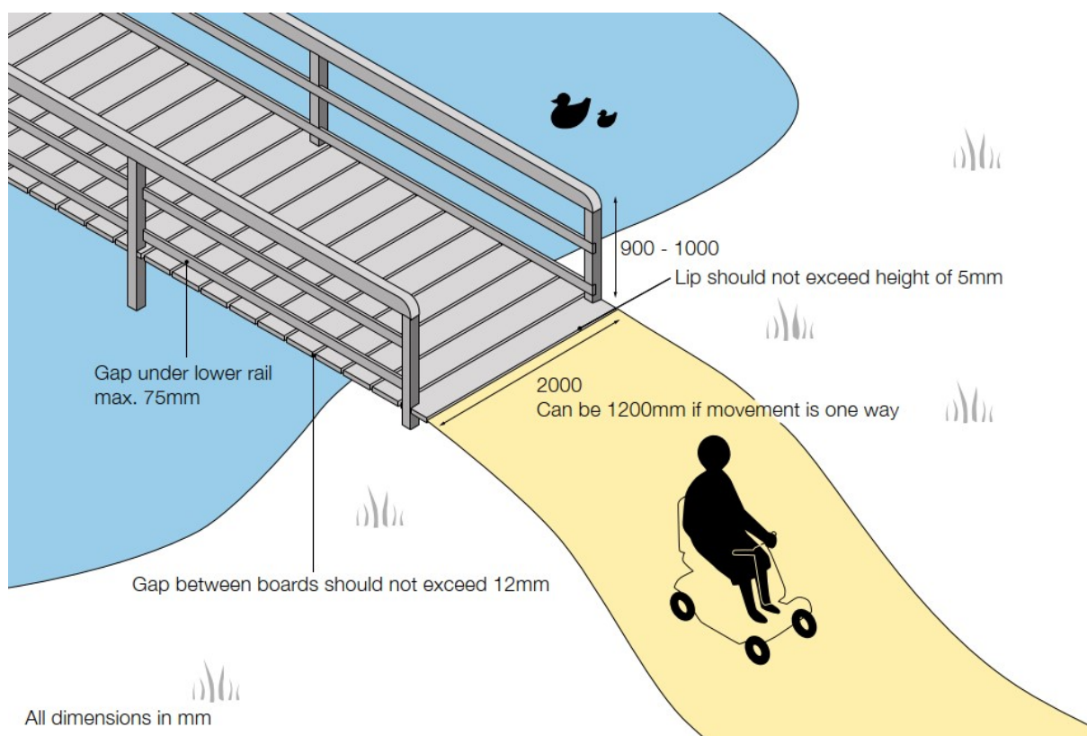
Figure 20: Rural bridge
