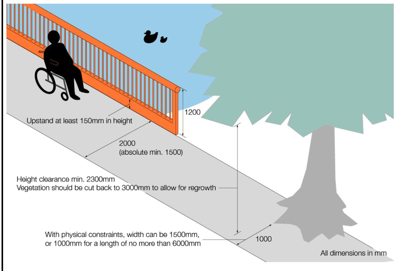
Figure 1: Footway widths, headroom requirements and guardrails
