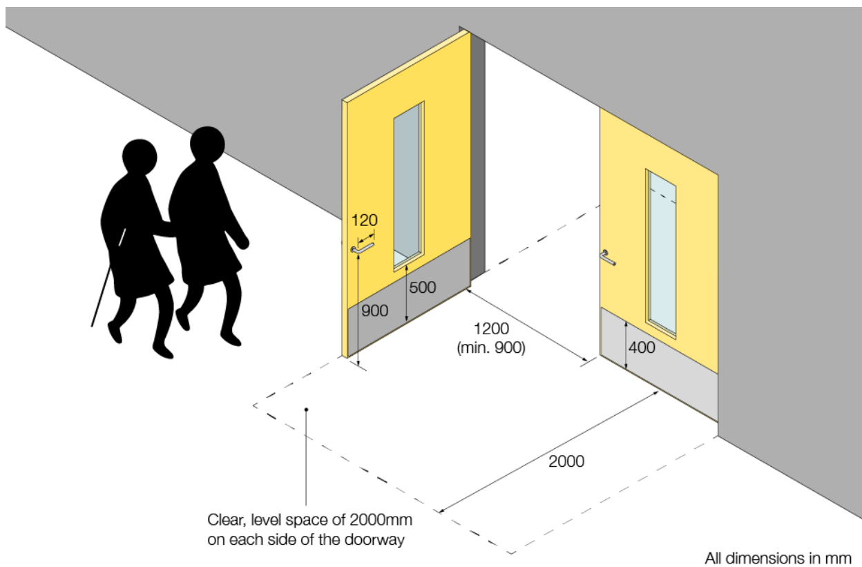
Figure 14: Manually operated doors
