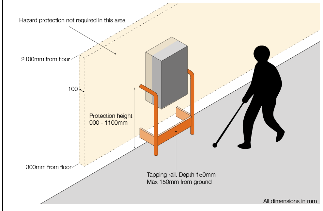
Figure 2: Low-level obstructions
