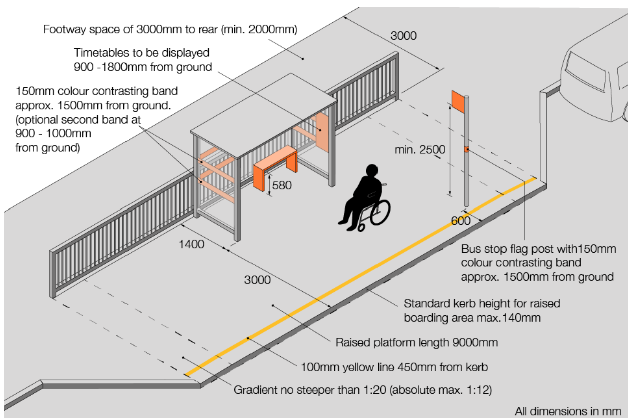
Figure 13: Bus stop
