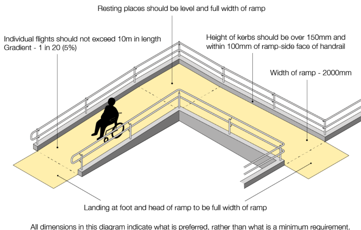
Figure 5: Ramps
