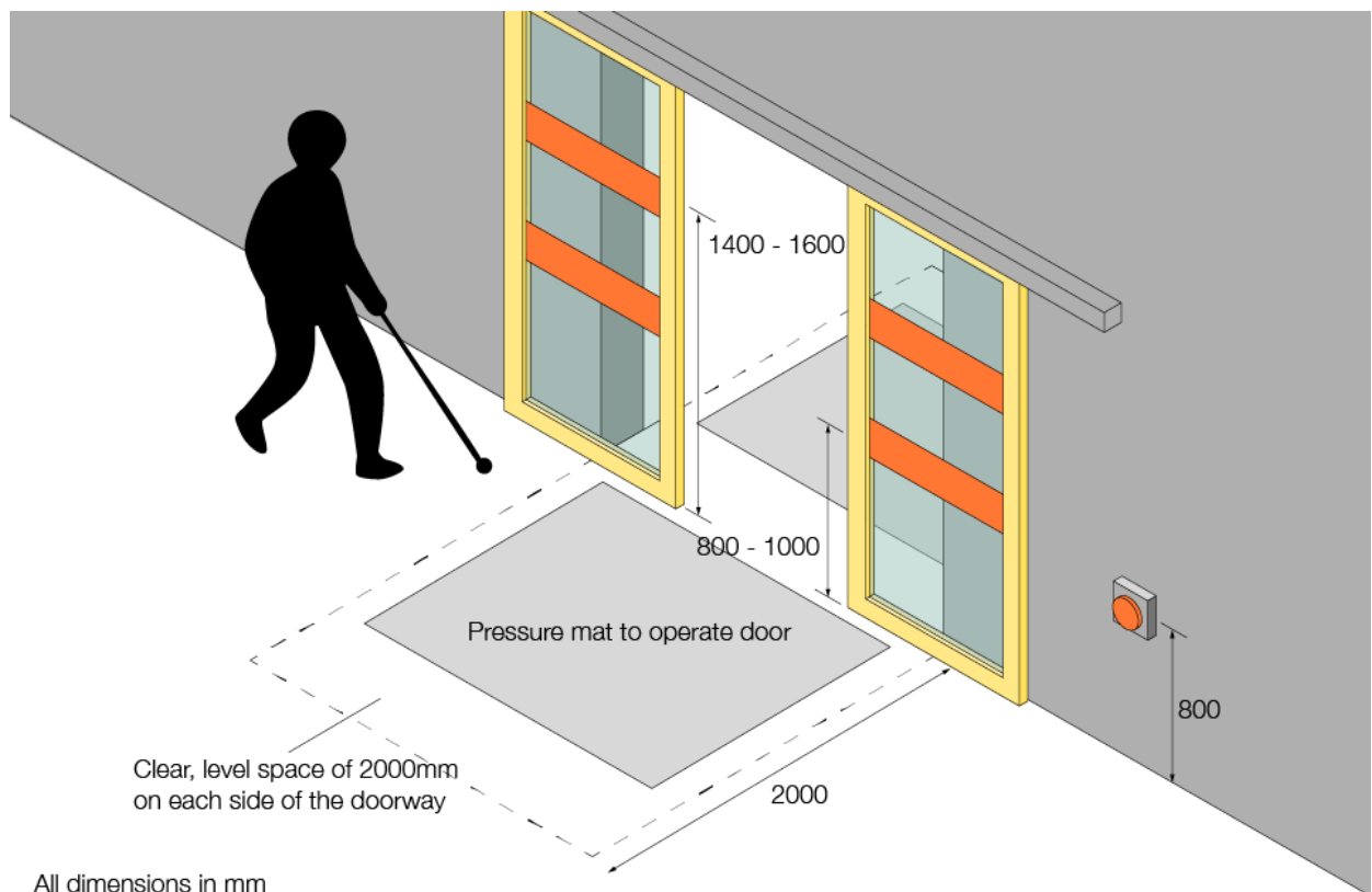
Figure 15: Automatic sliding doors
