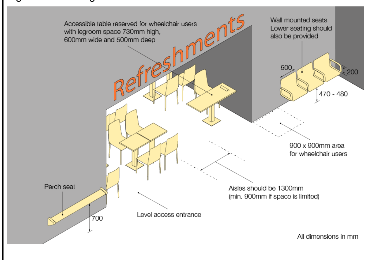
Figure 17: Waiting and refreshment facilities
