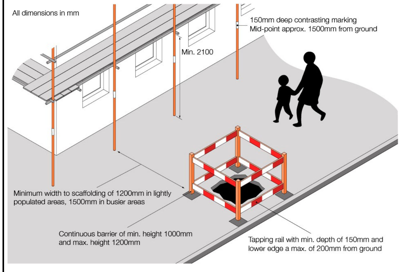
Figure 3: Street works protection
