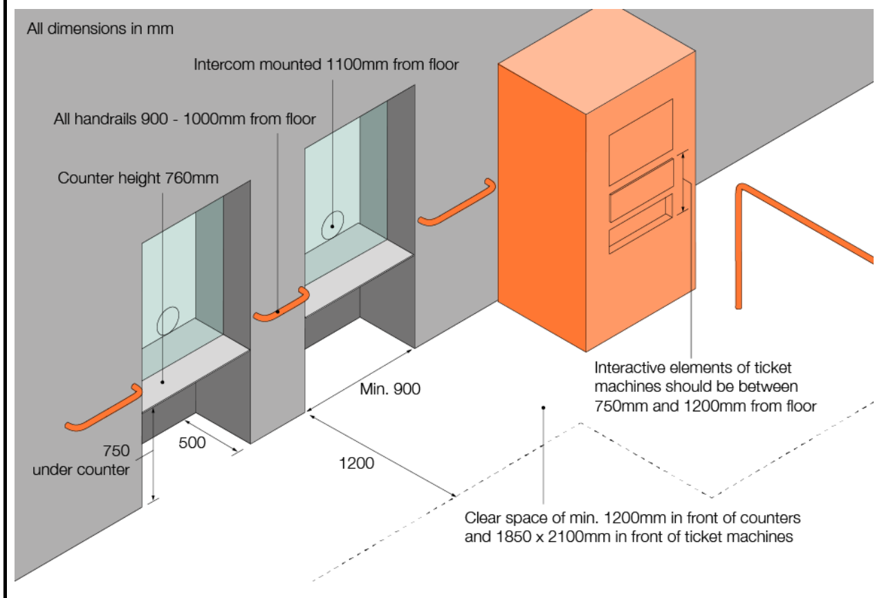
Figure 16: Ticketing / information counter
