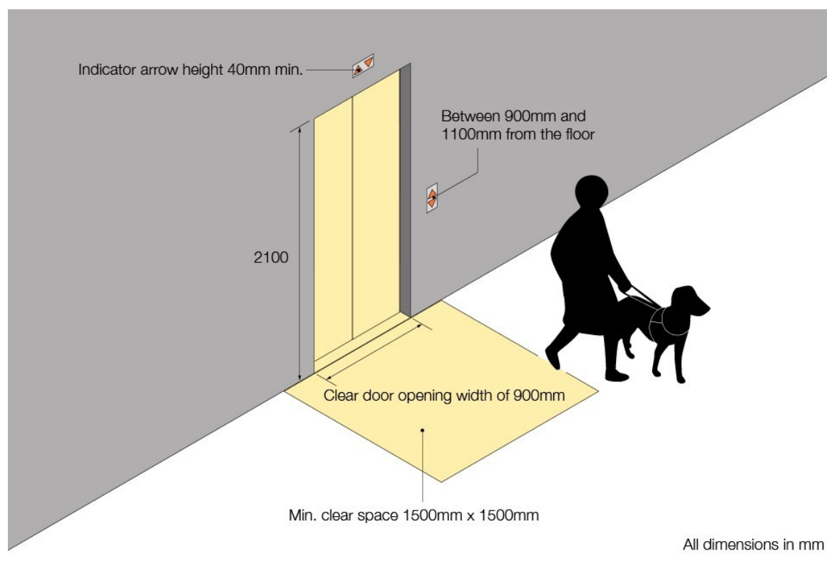
Figure 7: Lift exterior
