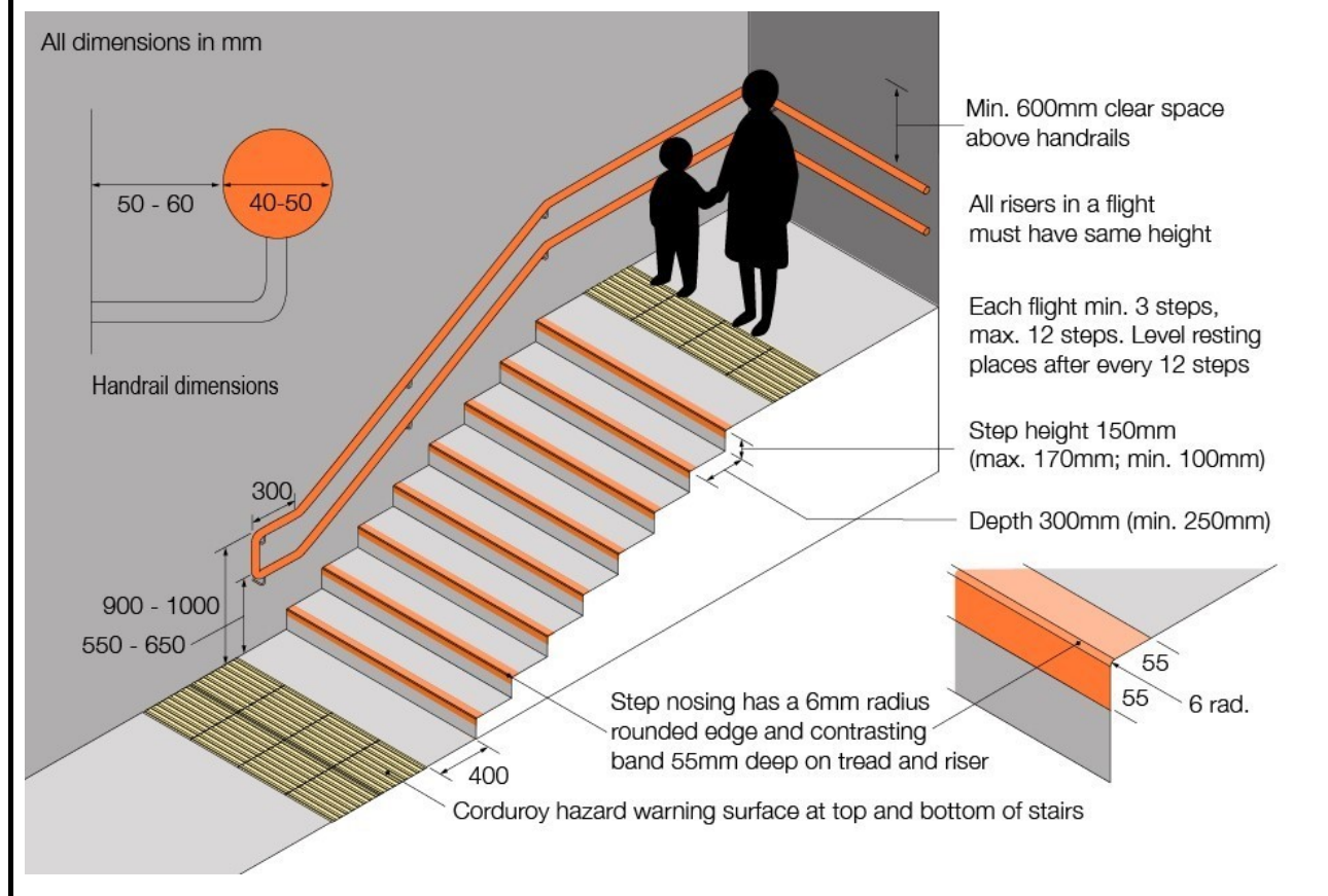
Figure 4: Stairs
