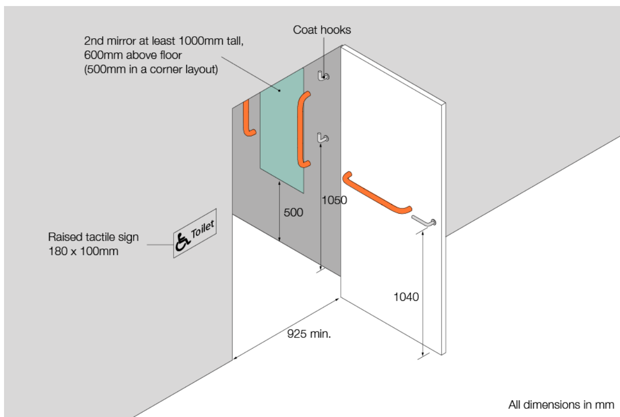
Figure 18: Toilet door
