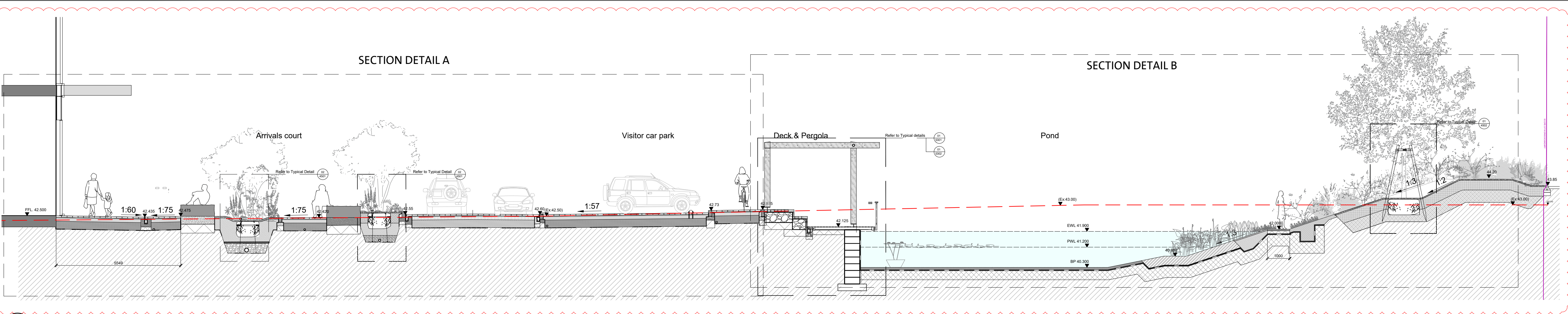
01 Section 1 - Arrival court and water pond scale 1:100 @ A1
