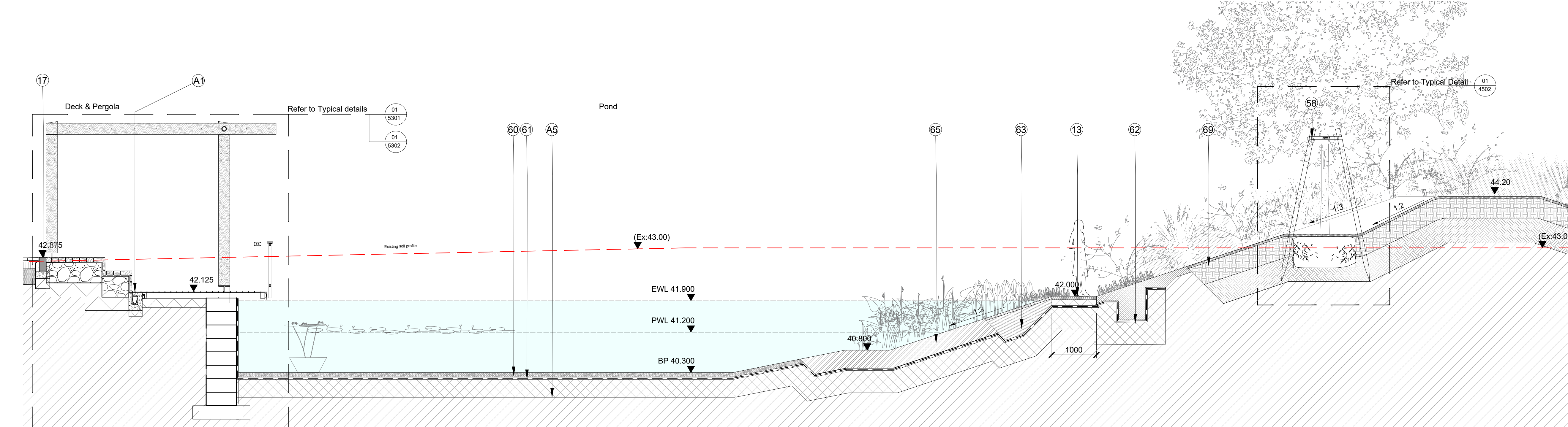
03 Section 1 - B scale 1:50 @ A1
