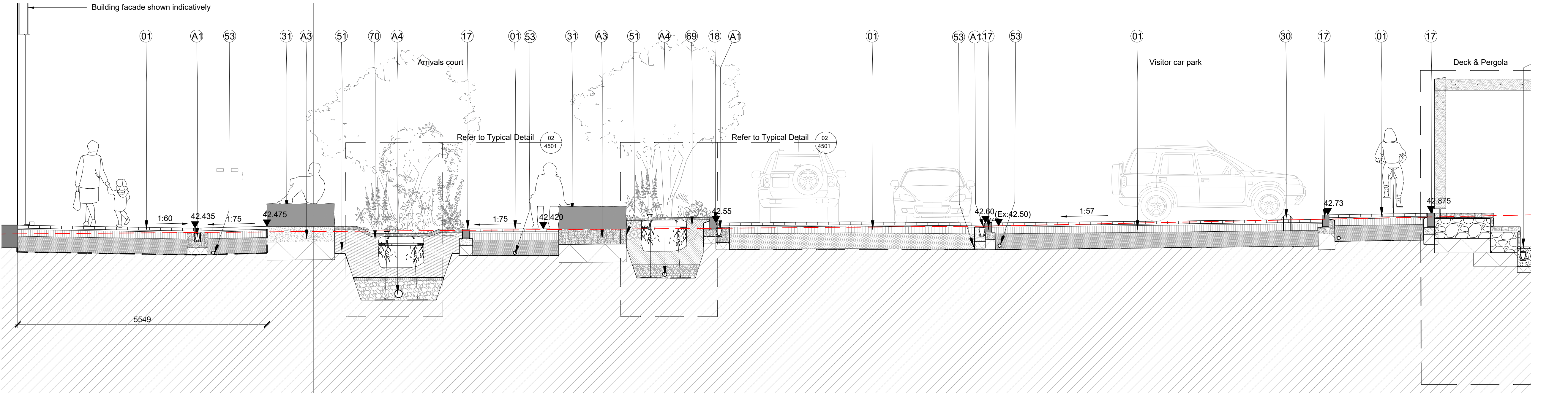
02 Section 1 - A scale 1:50 @ A1
