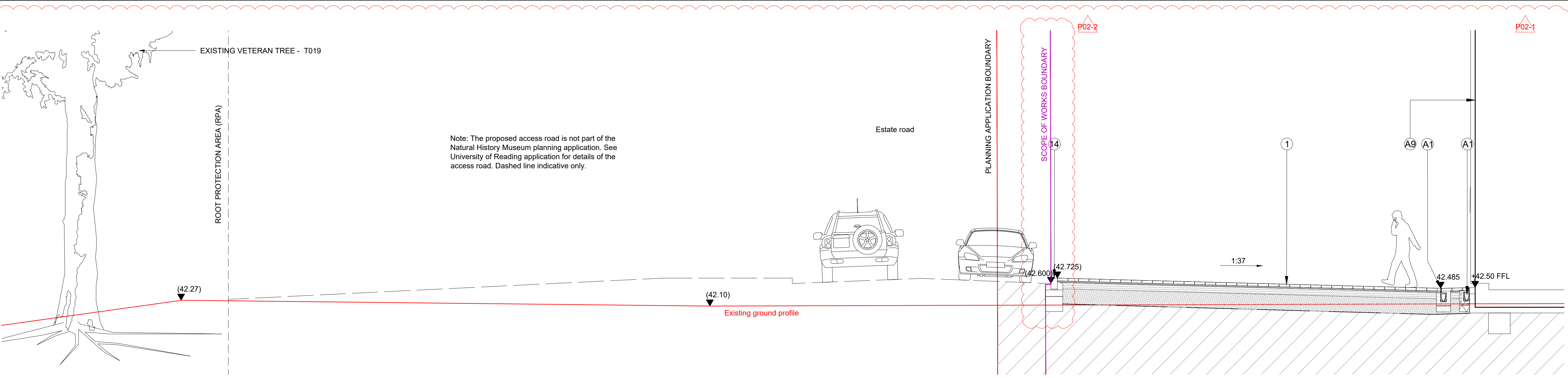
01 Section 9 - West Road scale 1:50 @ A1
