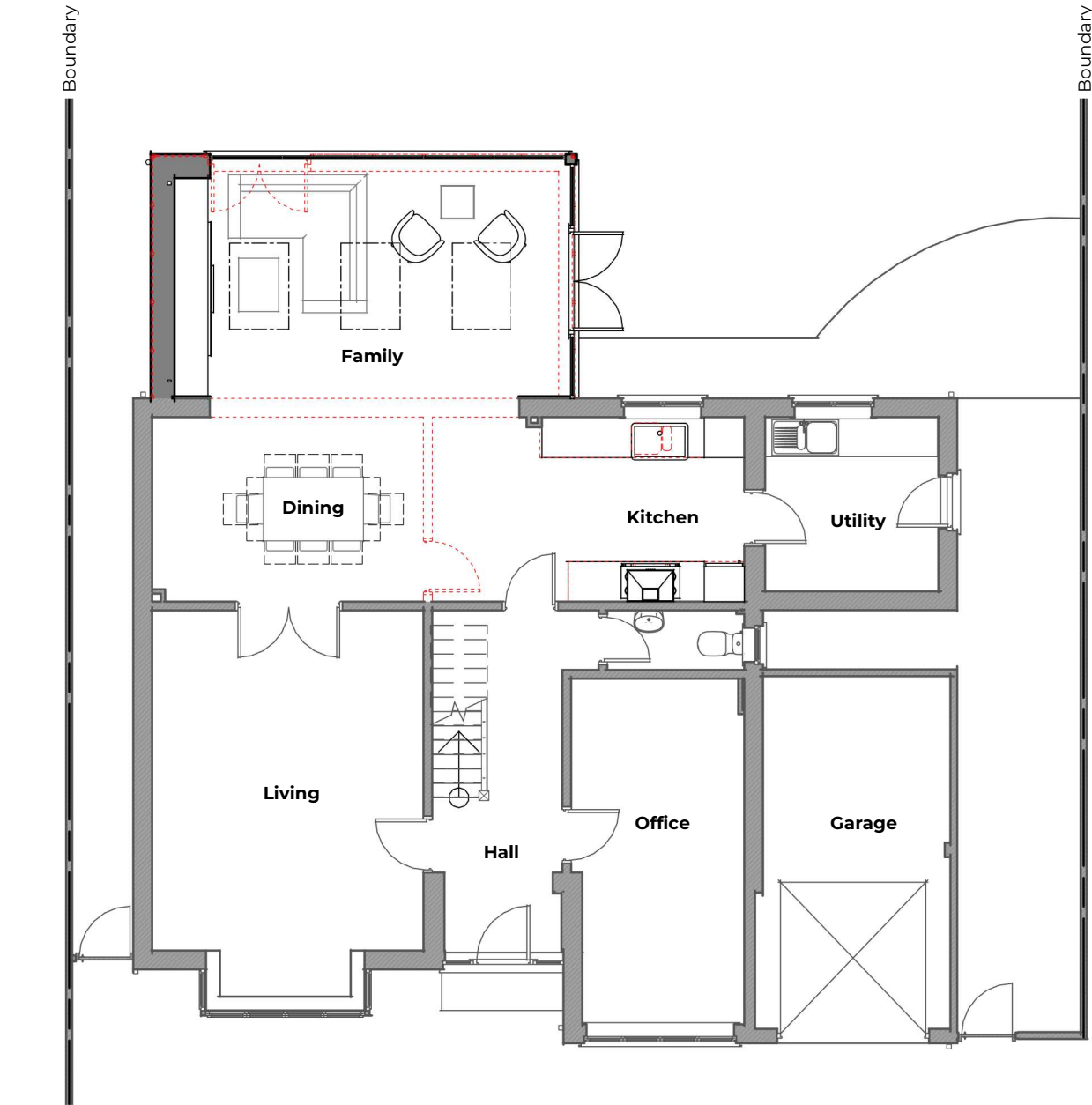
Proposed Ground Level Plan
