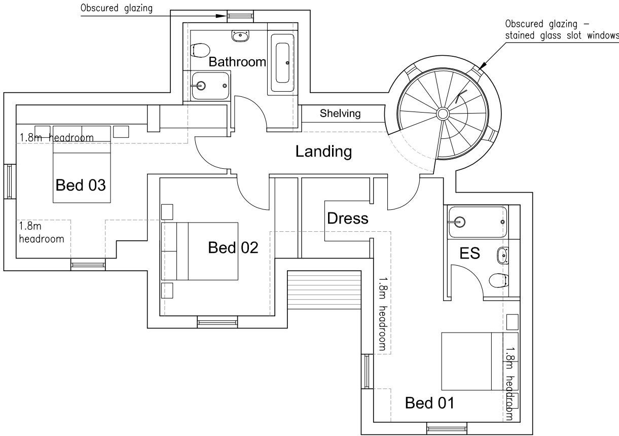
02 PROPOSED FIRST FLOOR PLAN
