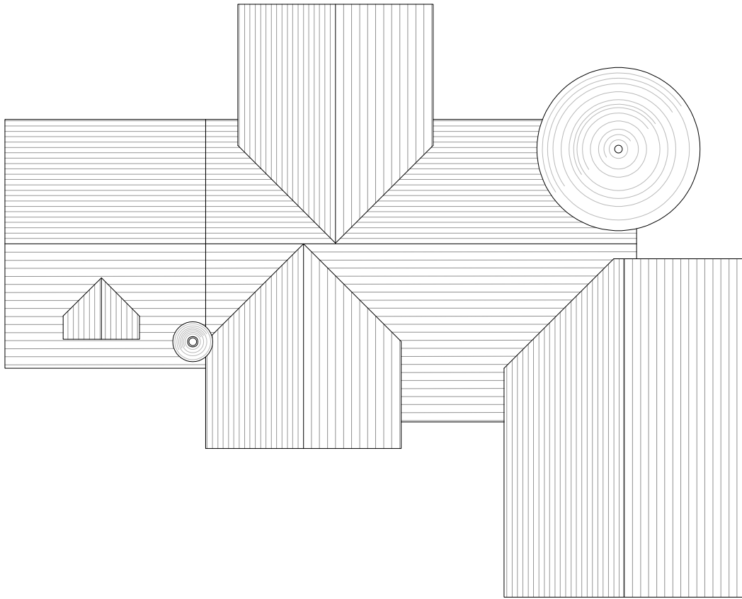
03 PROPOSED ROOF PLAN
