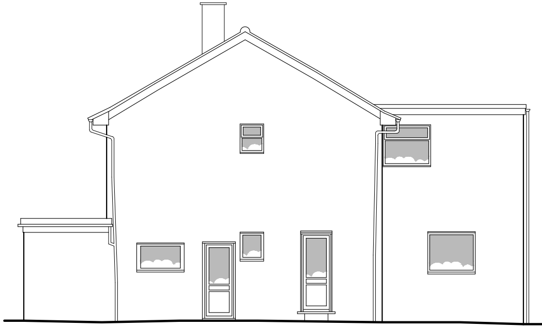
SIDE ELEVATION 1:100
