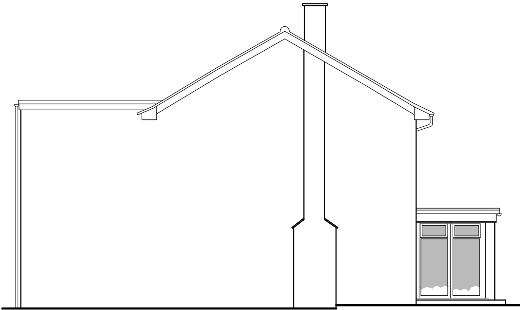
SIDE ELEVATION 1:100
