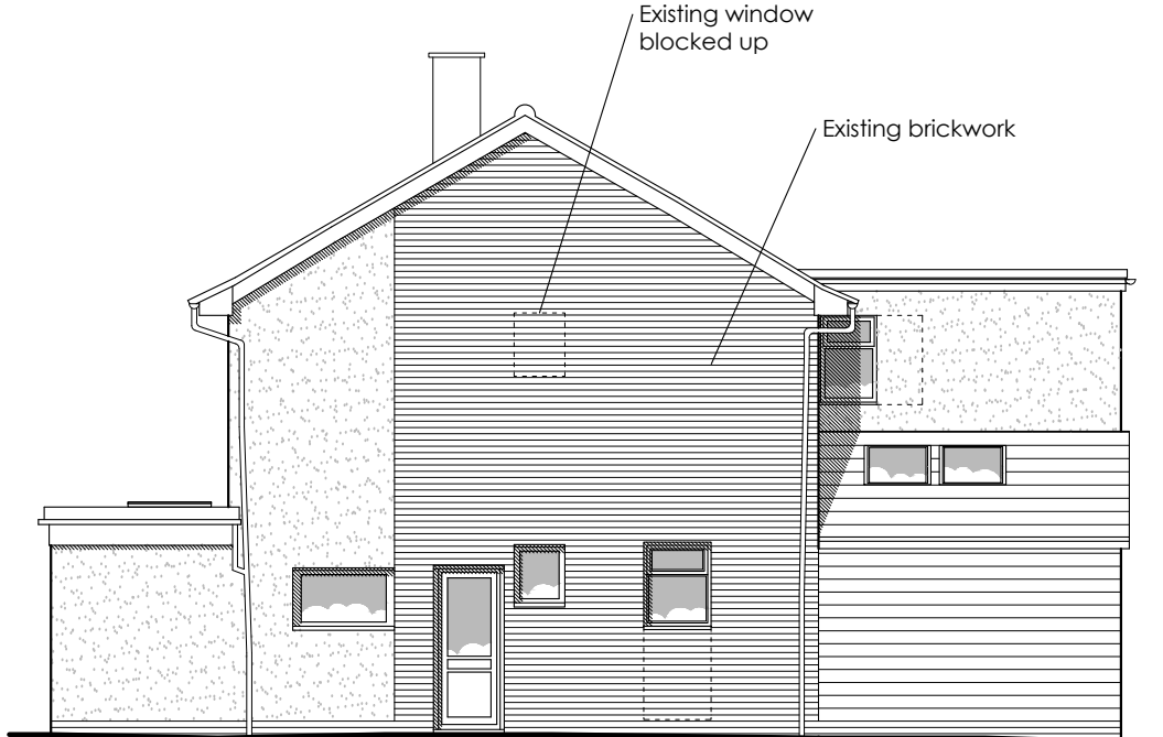
SIDE ELEVATION 1:100
