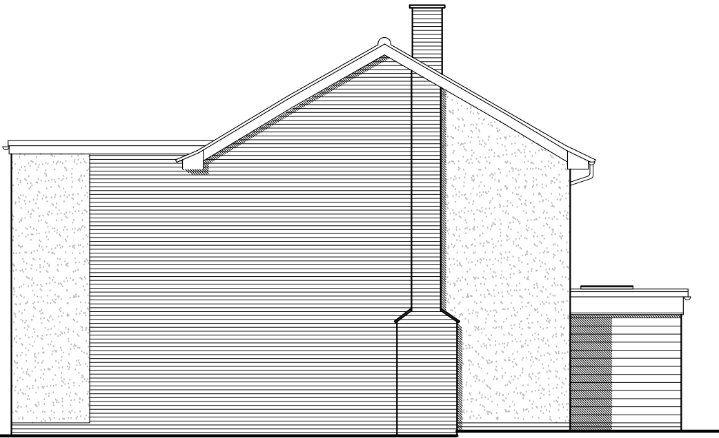
SIDE ELEVATION 1:100
