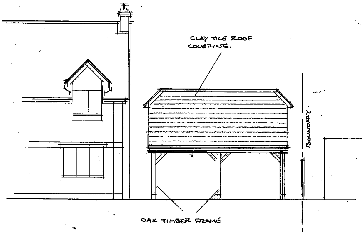
Front Elevation
