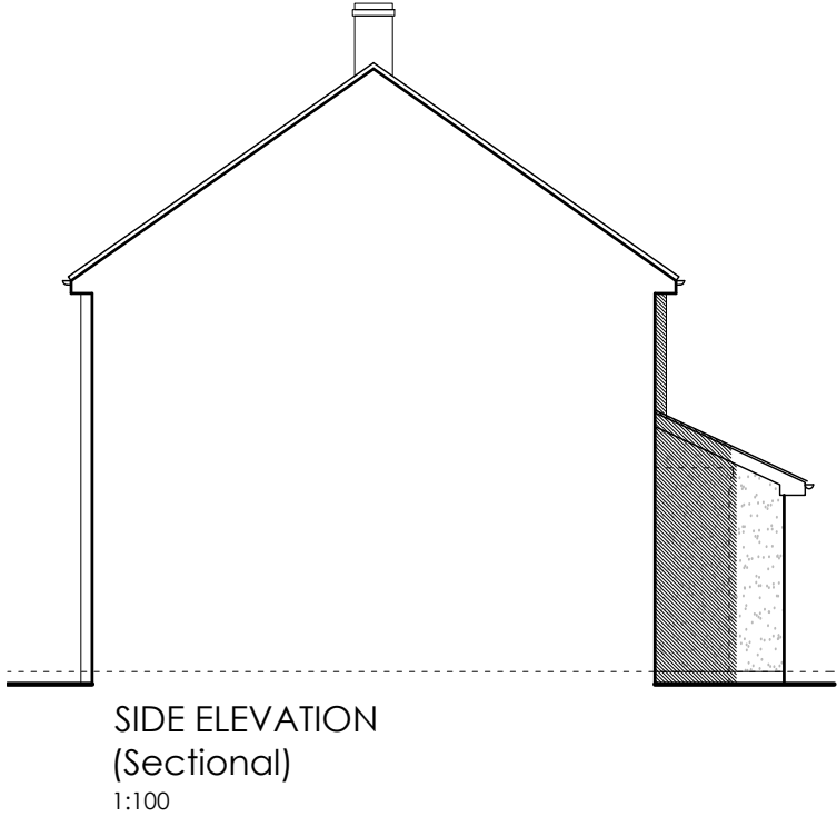
SIDE ELEVATION 1:100
