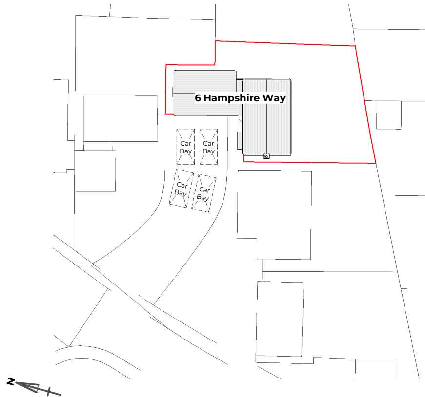
Existing Site Level Plan General Arrangement | Scale 1:500
