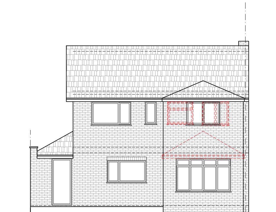
PROPOSED REAR SIDE ELEVATION
