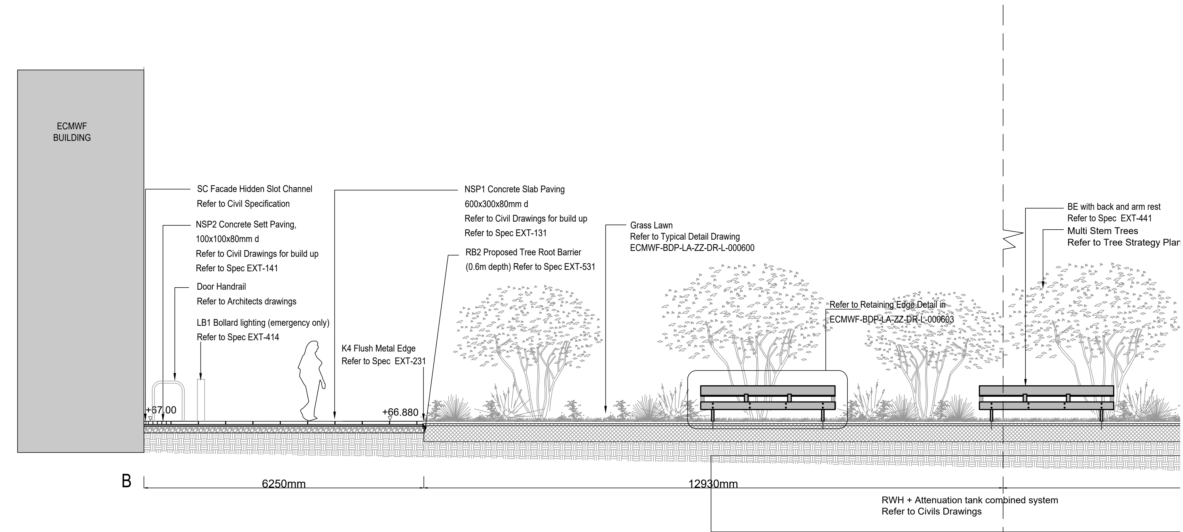
Landscape Section East - West 2 B-b
