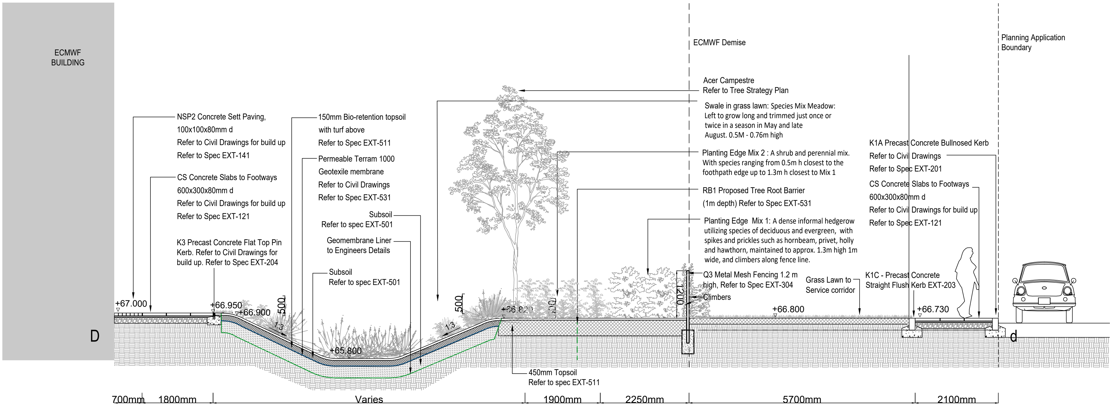
Landscape Section North - South 2 Dd
