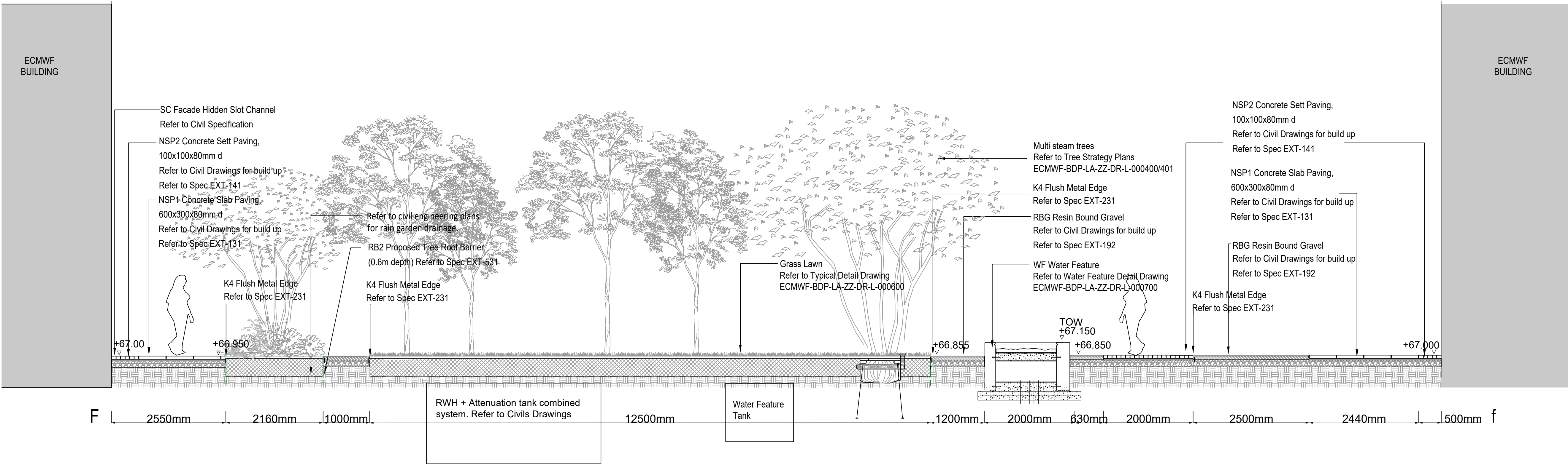
Landscape Section Courtyard - Ff
