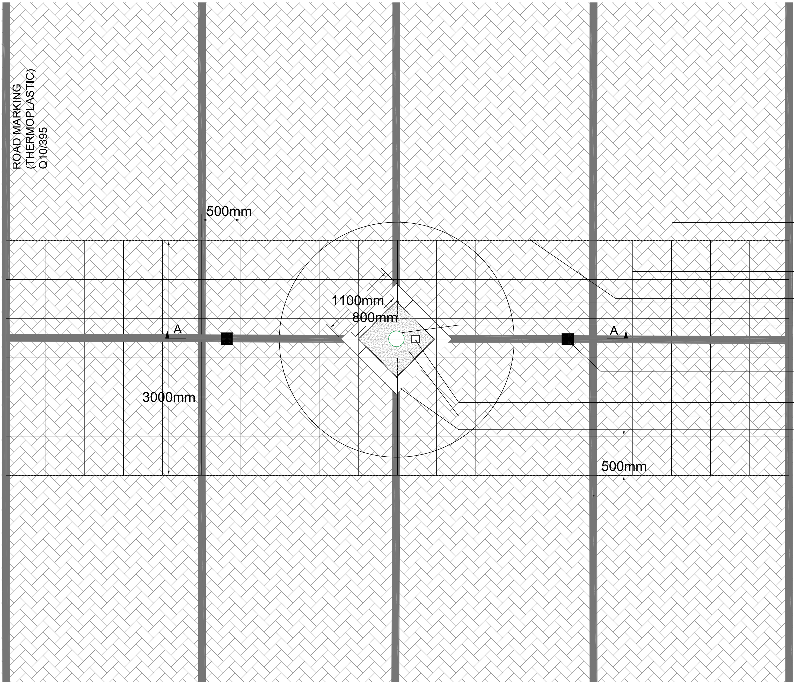
Car Park Tree Planting In Hard Landscape Plan Detail 1:25
