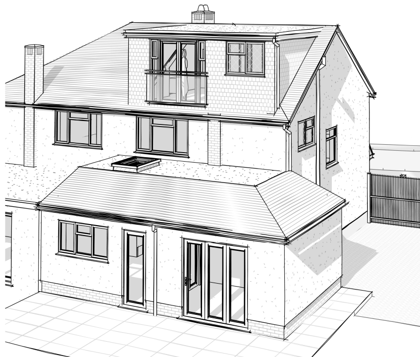
PROPOSED INDICATIVE 3D REAR ILLUSTRATION
