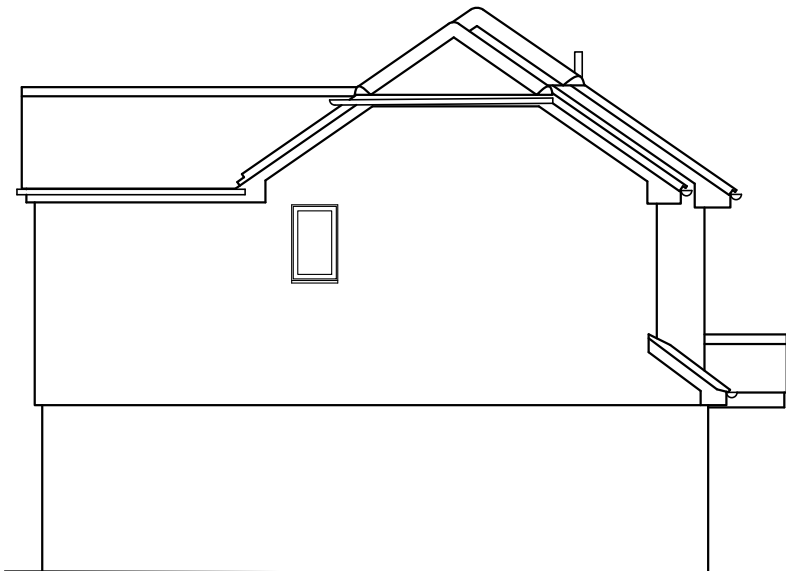
SIDE ELEVATION 1:100
