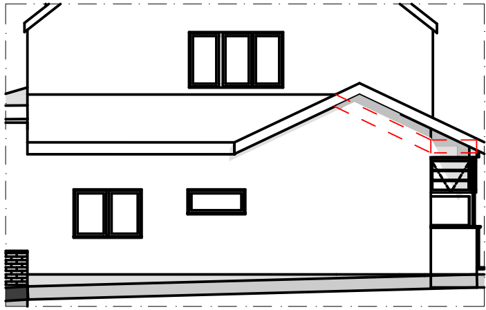
1:100 Proposed Side Elevation
