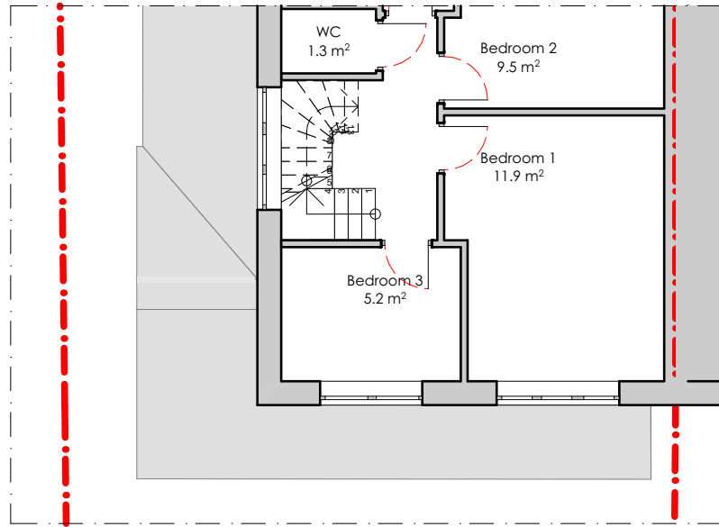
1:100 Proposed First Floor
