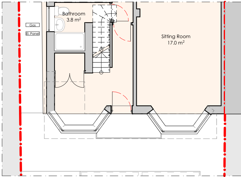
1:100 Proposed Ground Floor
