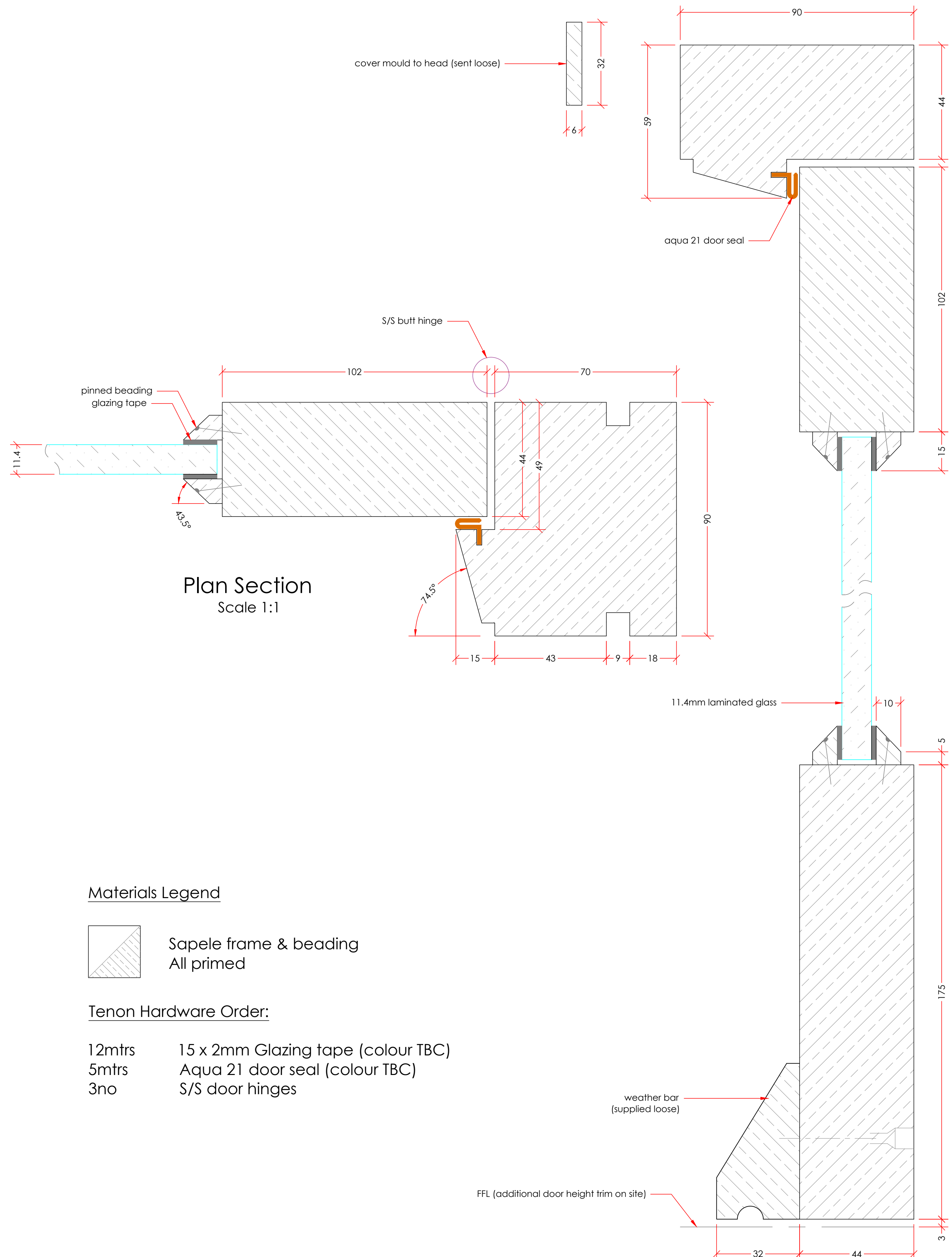
Height Section Scale 1:1
