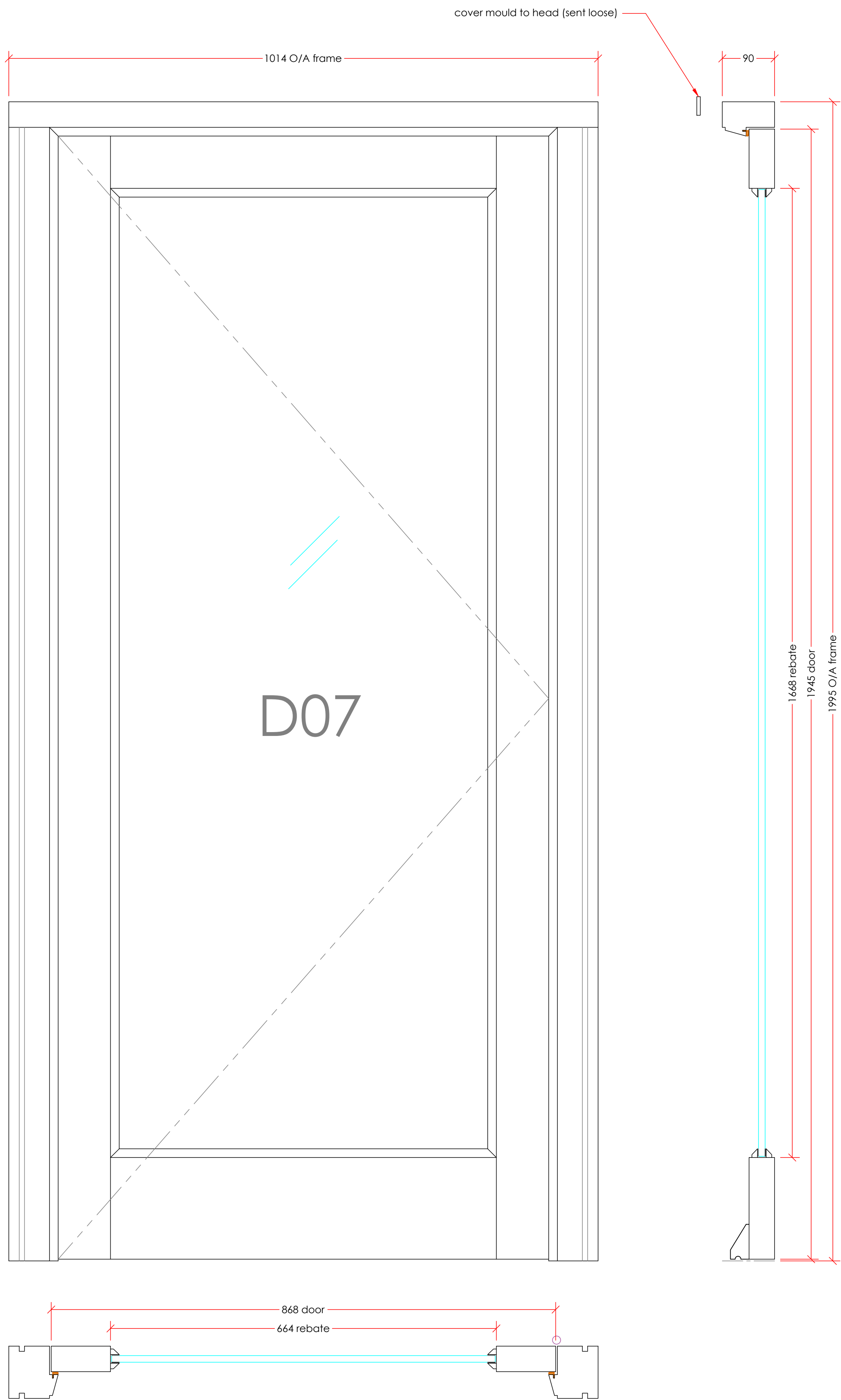
Elevations & Frame Dimensions Scale 1:5
