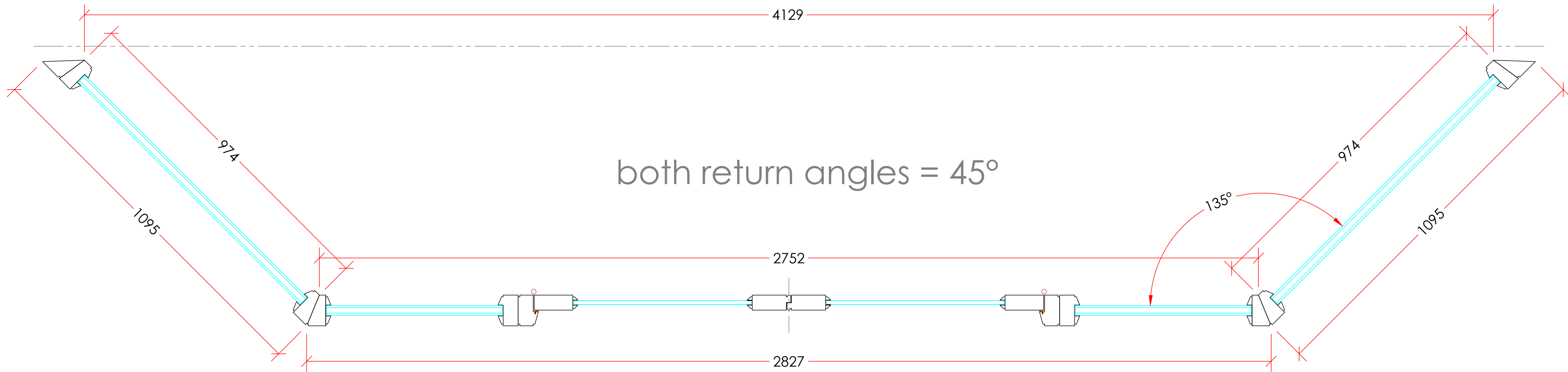
Assembled Plan View Scale 1:8
