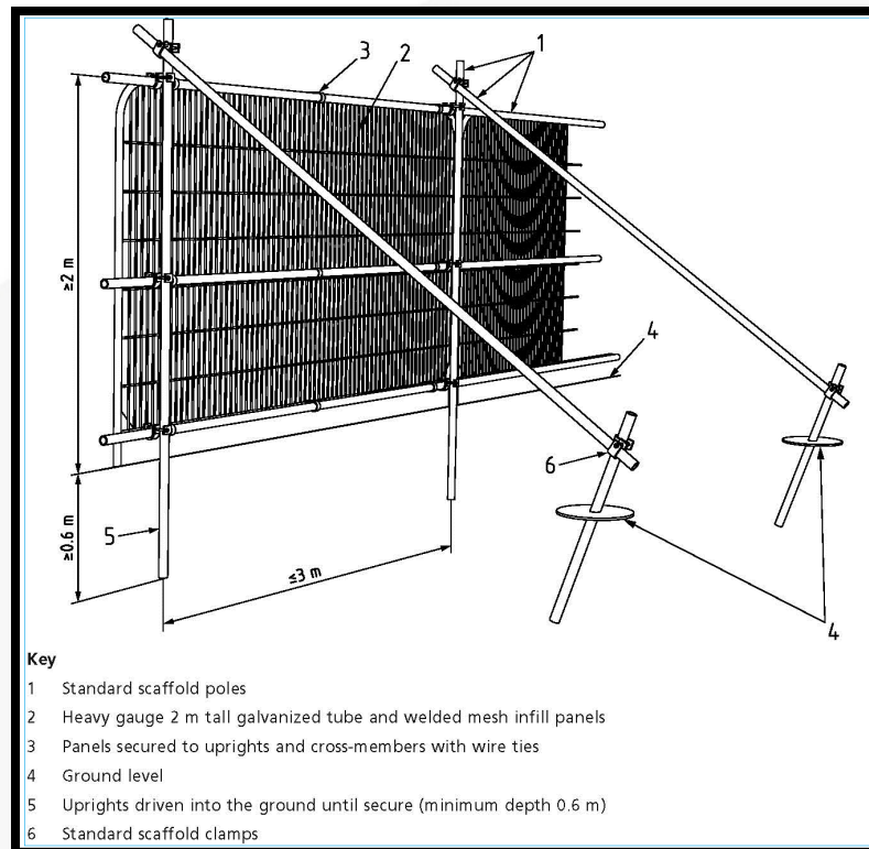
Figure 4: Default specification for protective barrier fencing (BS5837).
