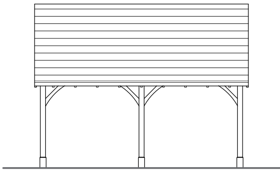
Elevation C
