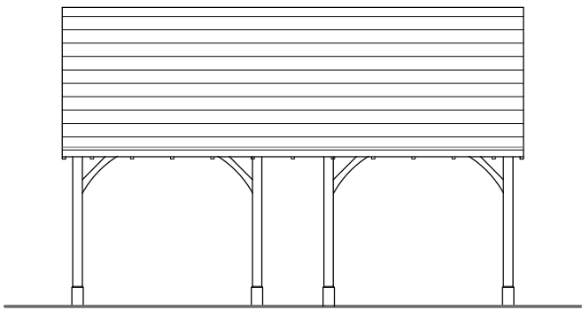
Elevation C
