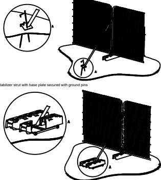
Figure 3 Examples of above-ground stabilizing systems
