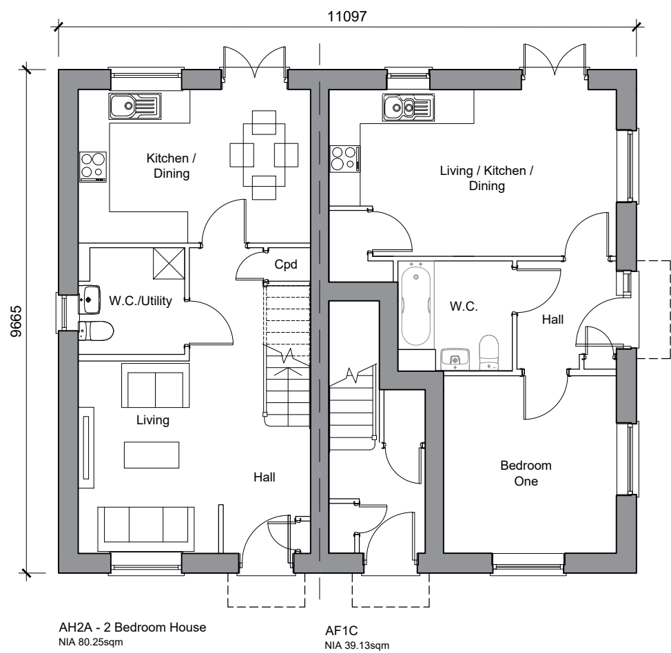
Ground Floor Plan Plots 192-193-194 Plots 153-154-155 (handed)
