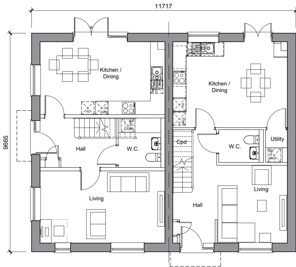
PH3C - 3 Bedroom House NIA 98.27sqm Ground Floor Plan Plot 228-229
