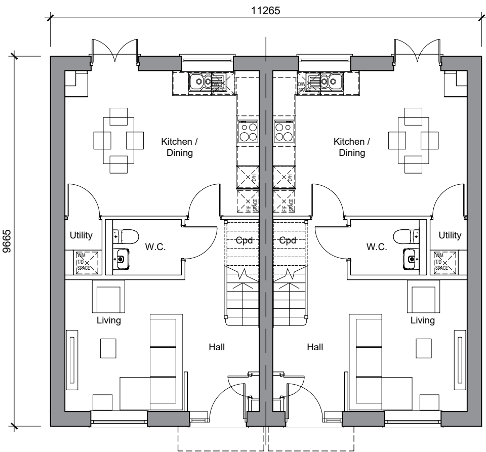
PH3B - 3 Bedroom House NIA 90.26sqm Ground Floor Plan Plots 129-130, 134-135, 145-146, 160-161, 164-165
