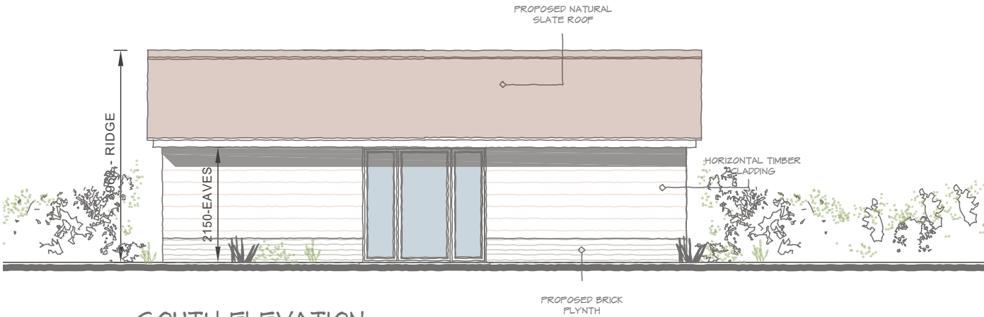
SOUTH ELEVATION
