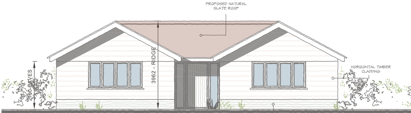
WEST ELEVATION
