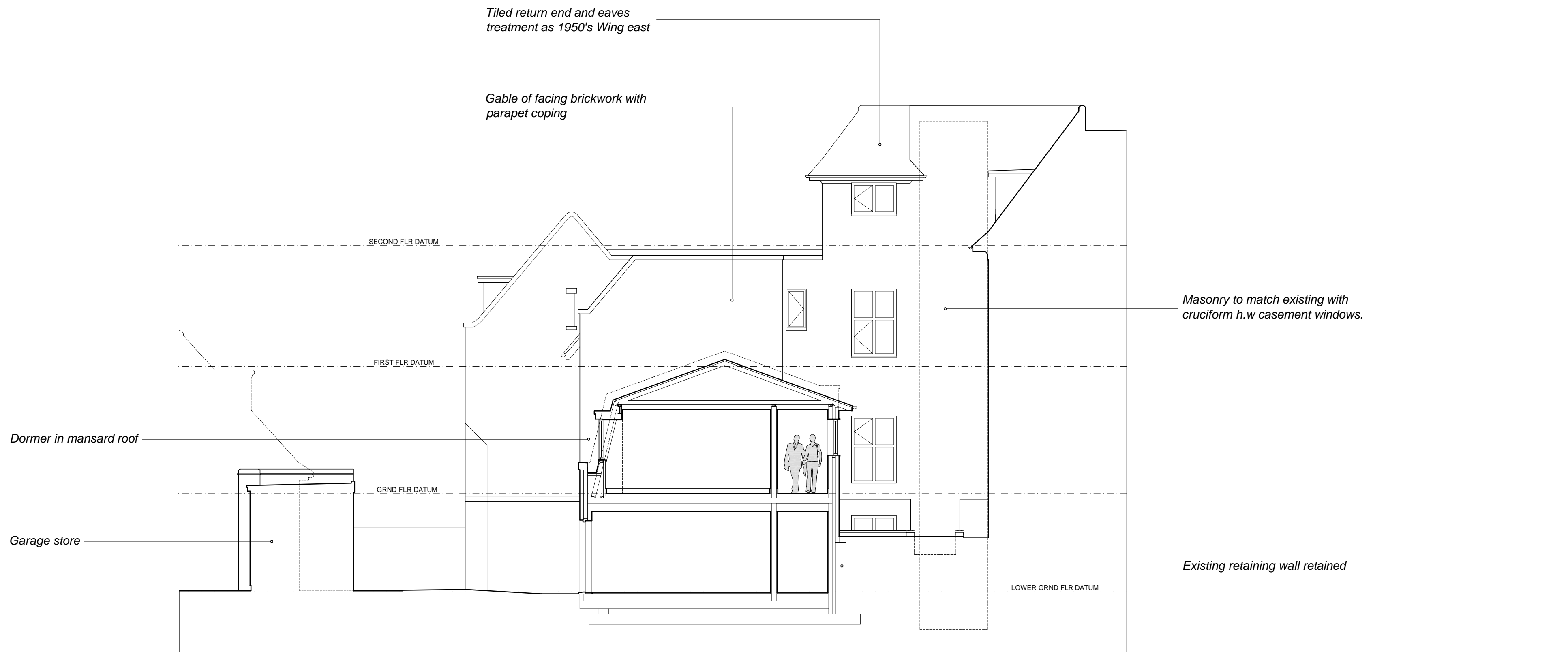
Section b (Proposed Link Wing)
