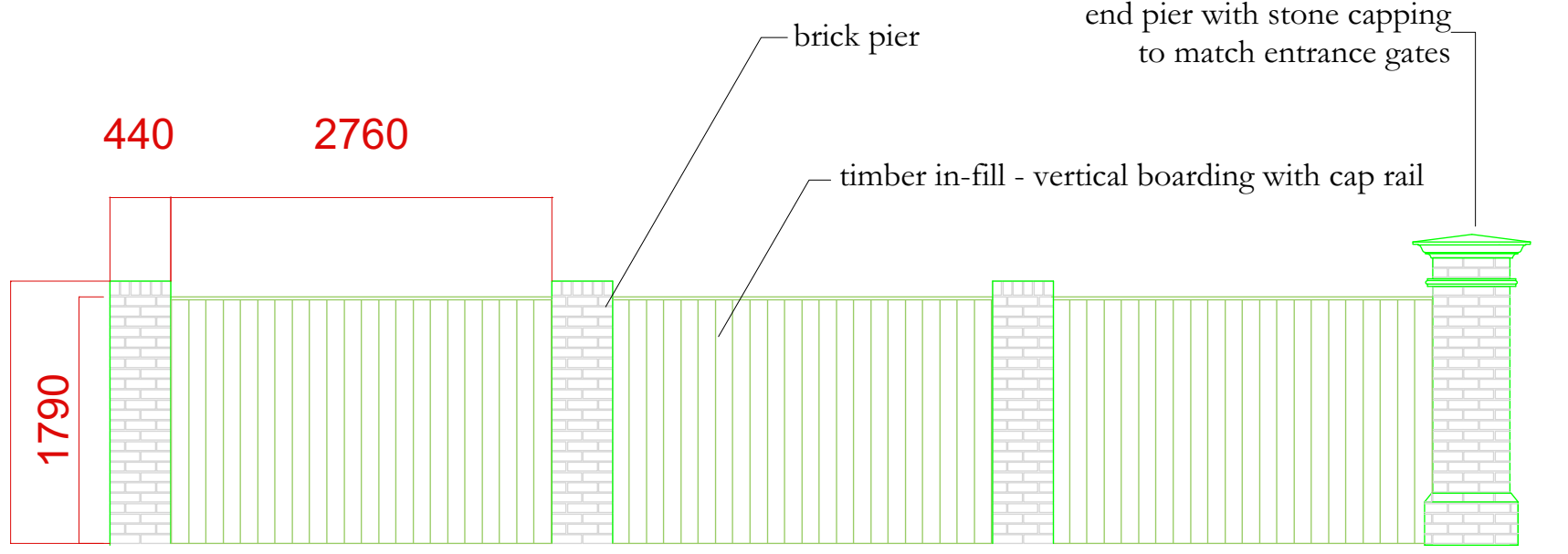
ELEVATION OF PROPOSED BOUNDARY WALL
