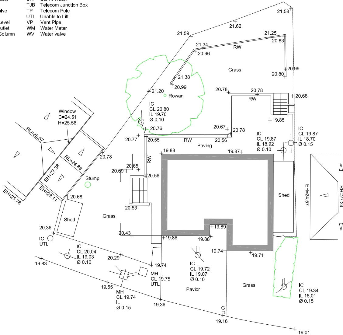
EXISTING BLOCK PLAN
