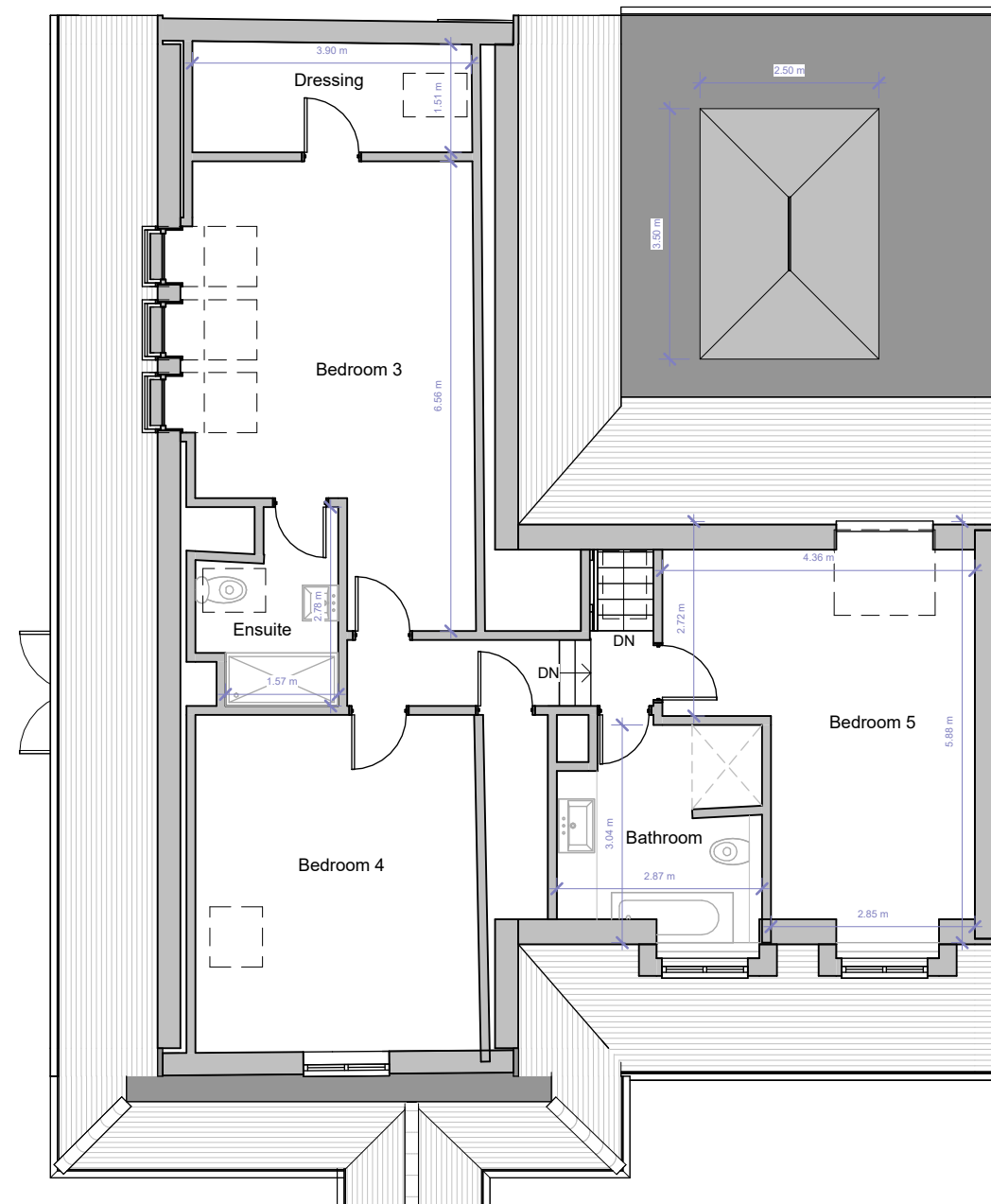
First Floor
