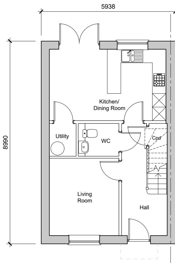
Ground Floor Plan 3-Bedroom House 86.00sqm / 925.69sqft GIA (to include) Plots - 5, 10, 12, 14, 28, 30, 32, 37, 46 Handed - 11, 13, 15, 16, 29, 31, 33, 39, 43, 47, 51, 54, 55
